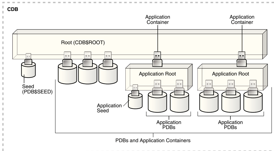
Figure 36-2 Application Containers in a CDB
