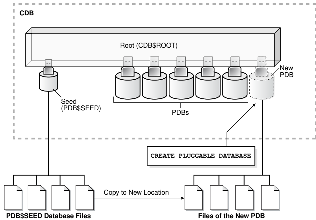
Figure 38-2 Create a PDB in the CDB Root Using the CDB Seed Files
