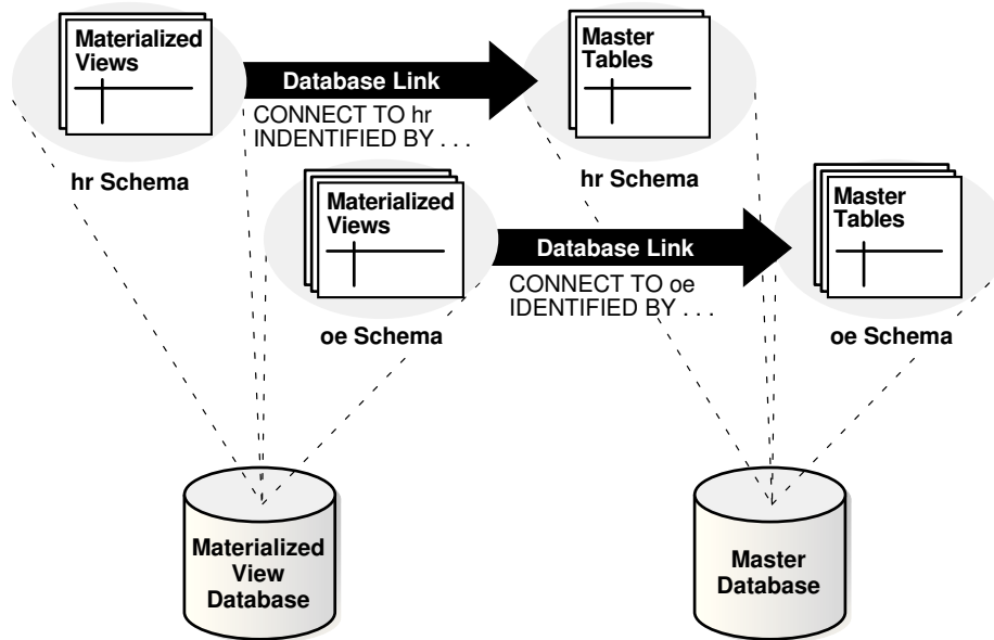
Figure 60-1 Recommended Schema and Database Link Configuration
