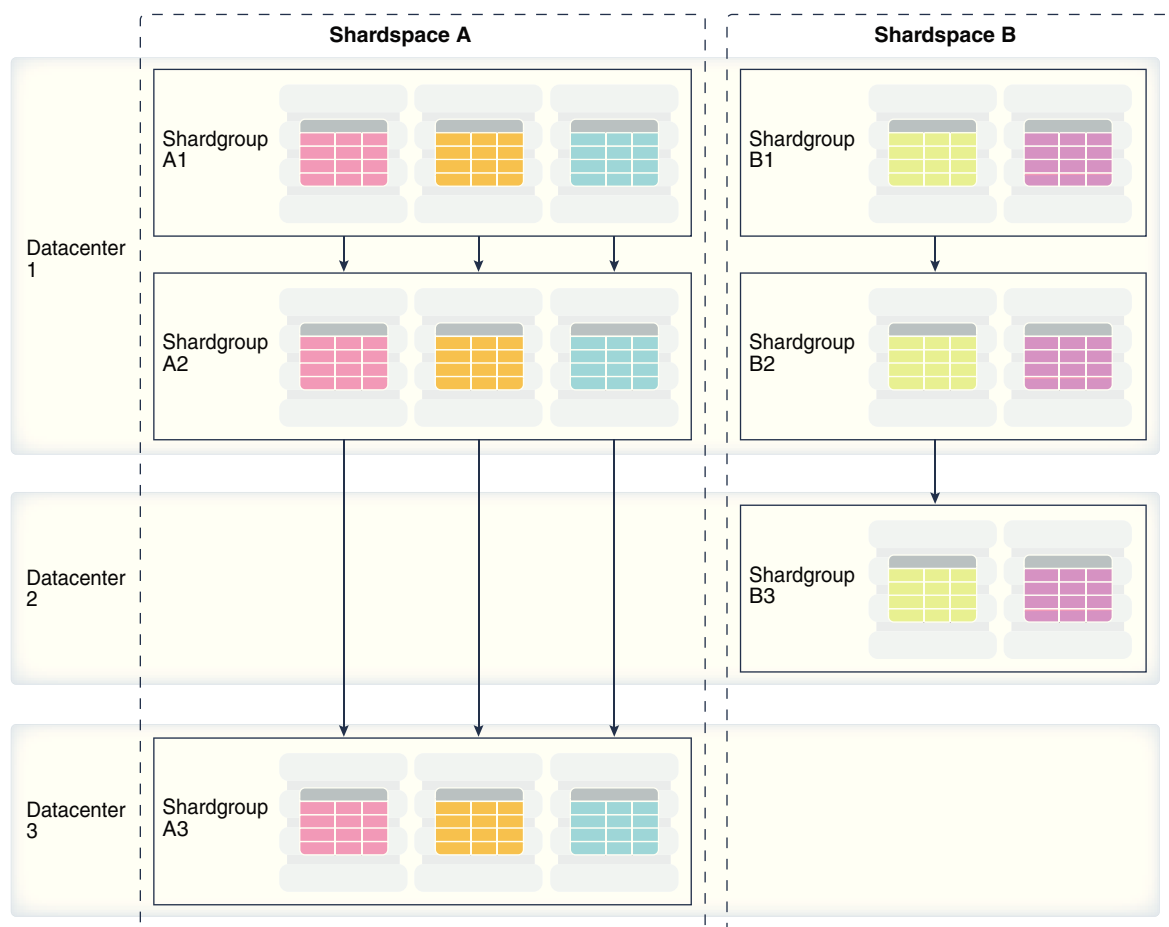
Figure 55-2 Composite Sharding with Data Guard Replication
