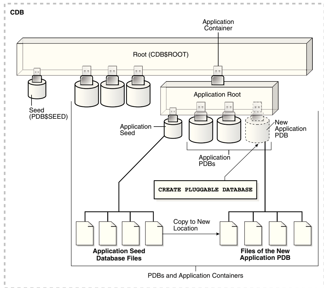
Figure 38-3 Create a PDB in an Application Root Using the Application Seed Files
