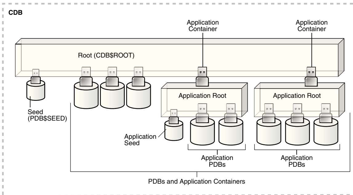
Figure 37-3 Application Containers in a CDB
