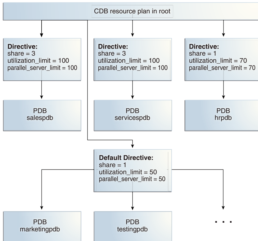
Figure 46-3 Default Directive in a CDB Resource Plan
