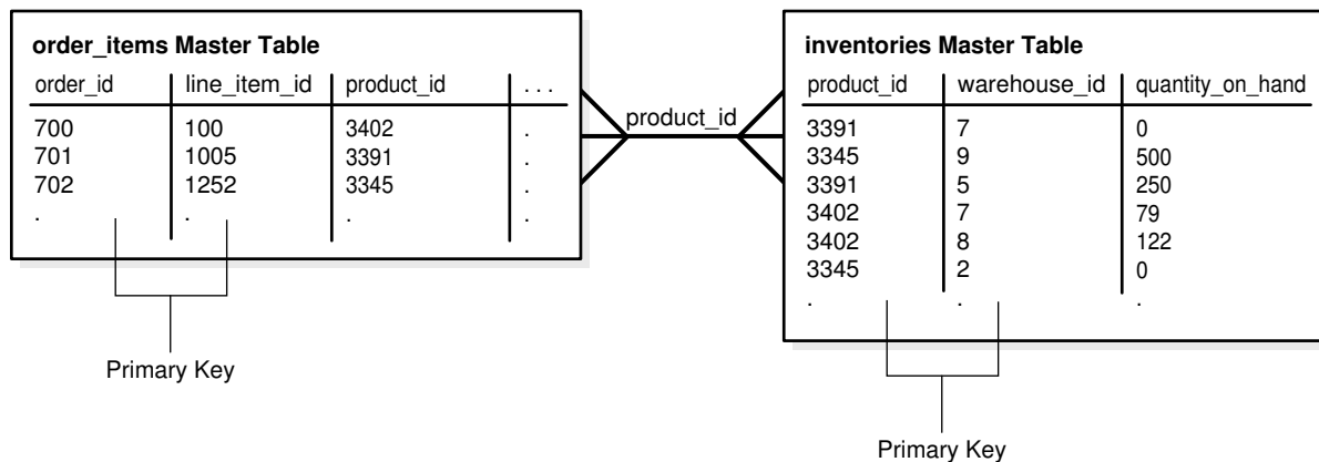
Figure 58-5 Row Subsetting with Many to Many Subqueries
