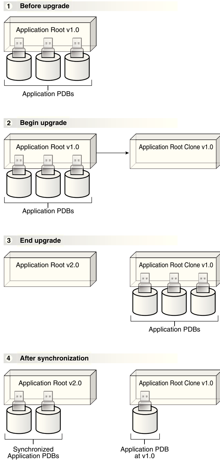
Figure 44-1 Upgrading Applications in an Application Container
