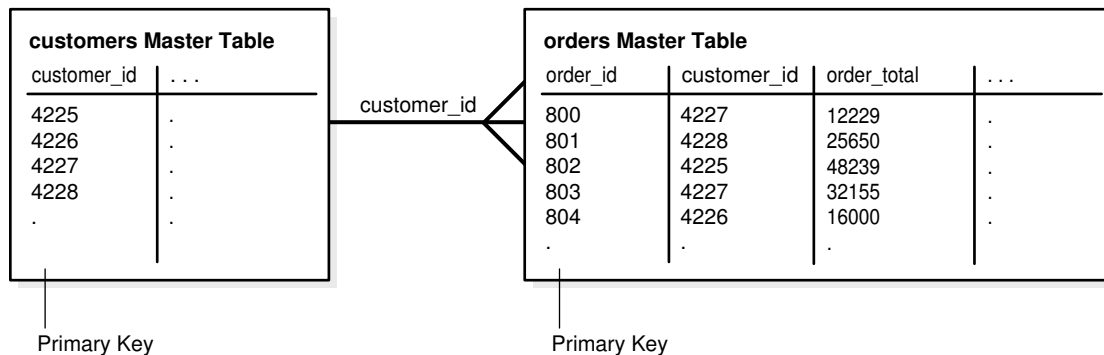
Figure 58-4 Row Subsetting with One to Many Subqueries
