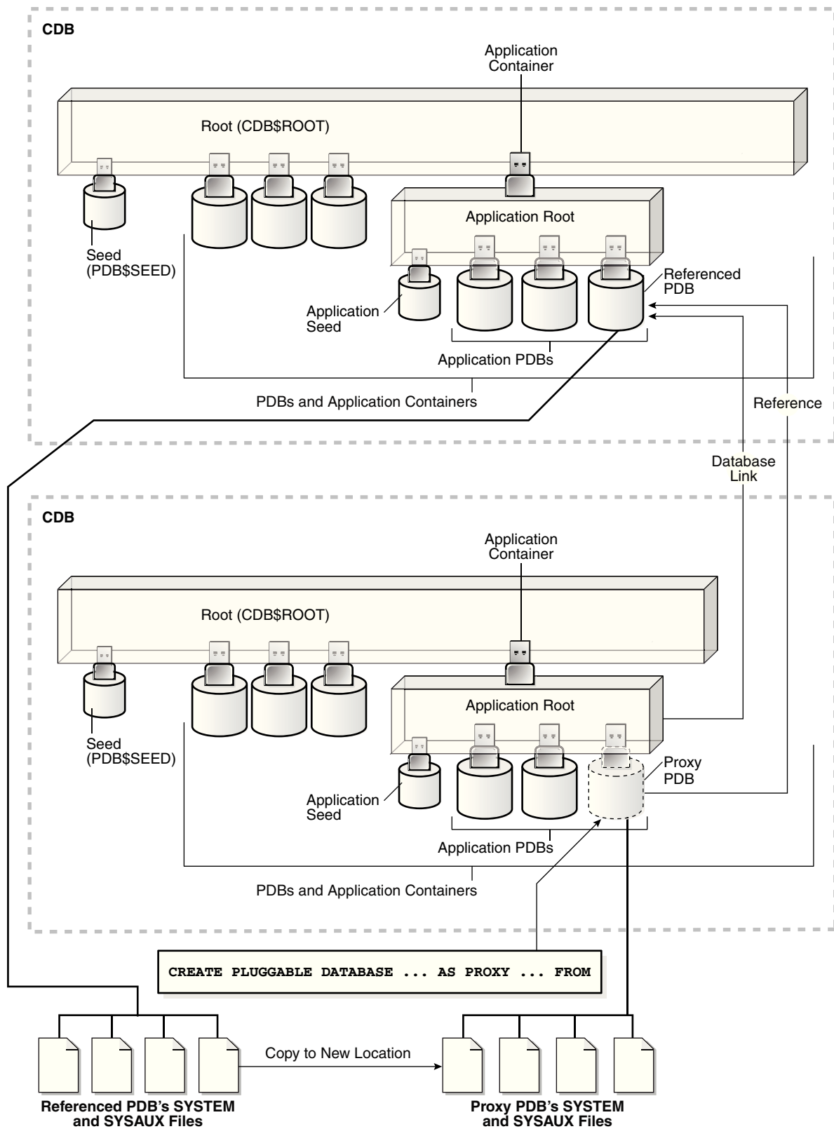
Figure 38-13 Create a Remote Proxy PDB in an Application Container
