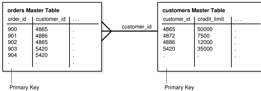
Figure 58-3 Row Subsetting with Many to One Subqueries
