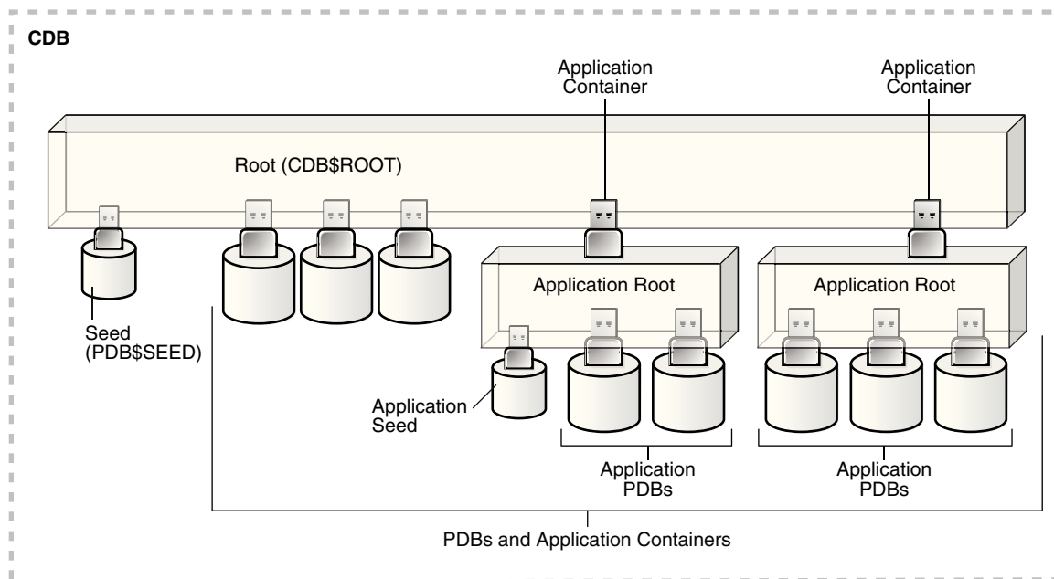
Figure 36-6 A CDB with PDBs, Application Containers, and Application PDBs
