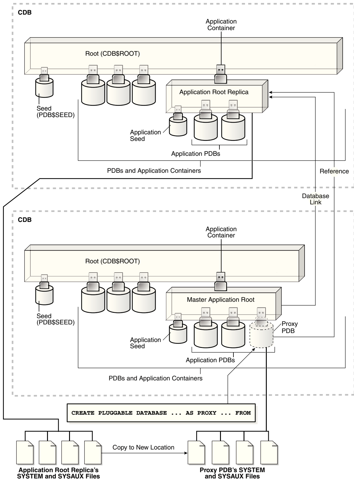
Figure 44-2 Synchronizing an Application Root Replica with a Proxy PDB
