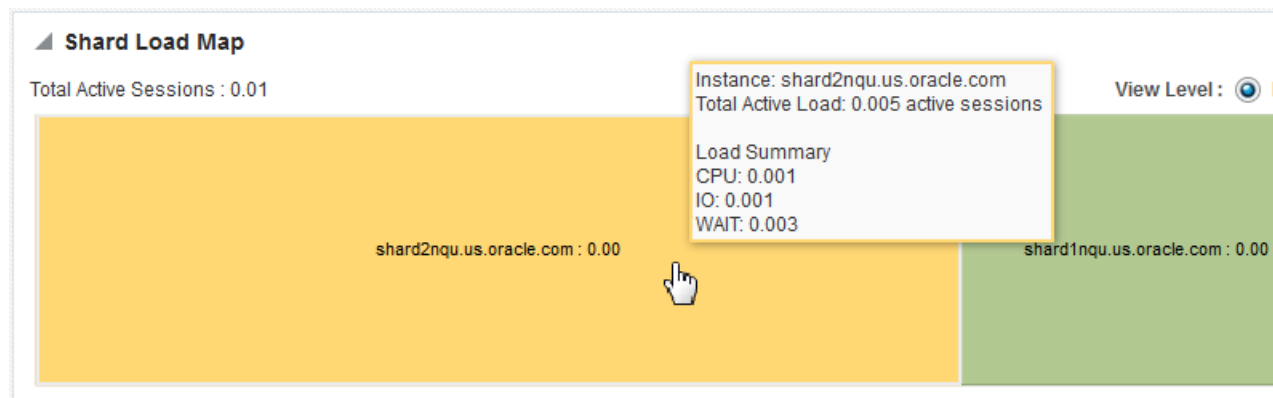
Figure 57-3 Sharded Database Shard Load Map
