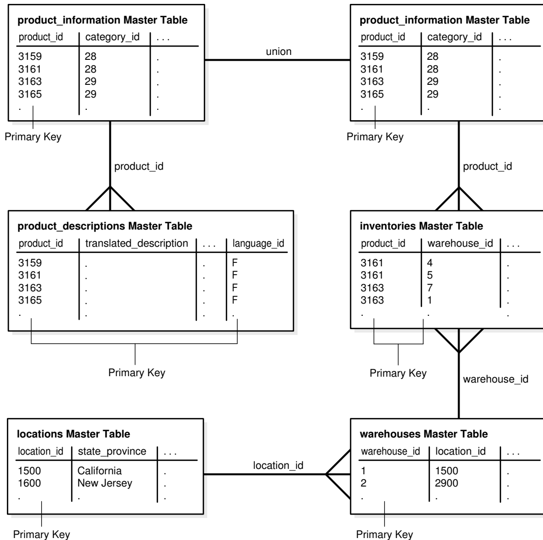
Figure 58-6 Row Subsetting with Subqueries and Unions
