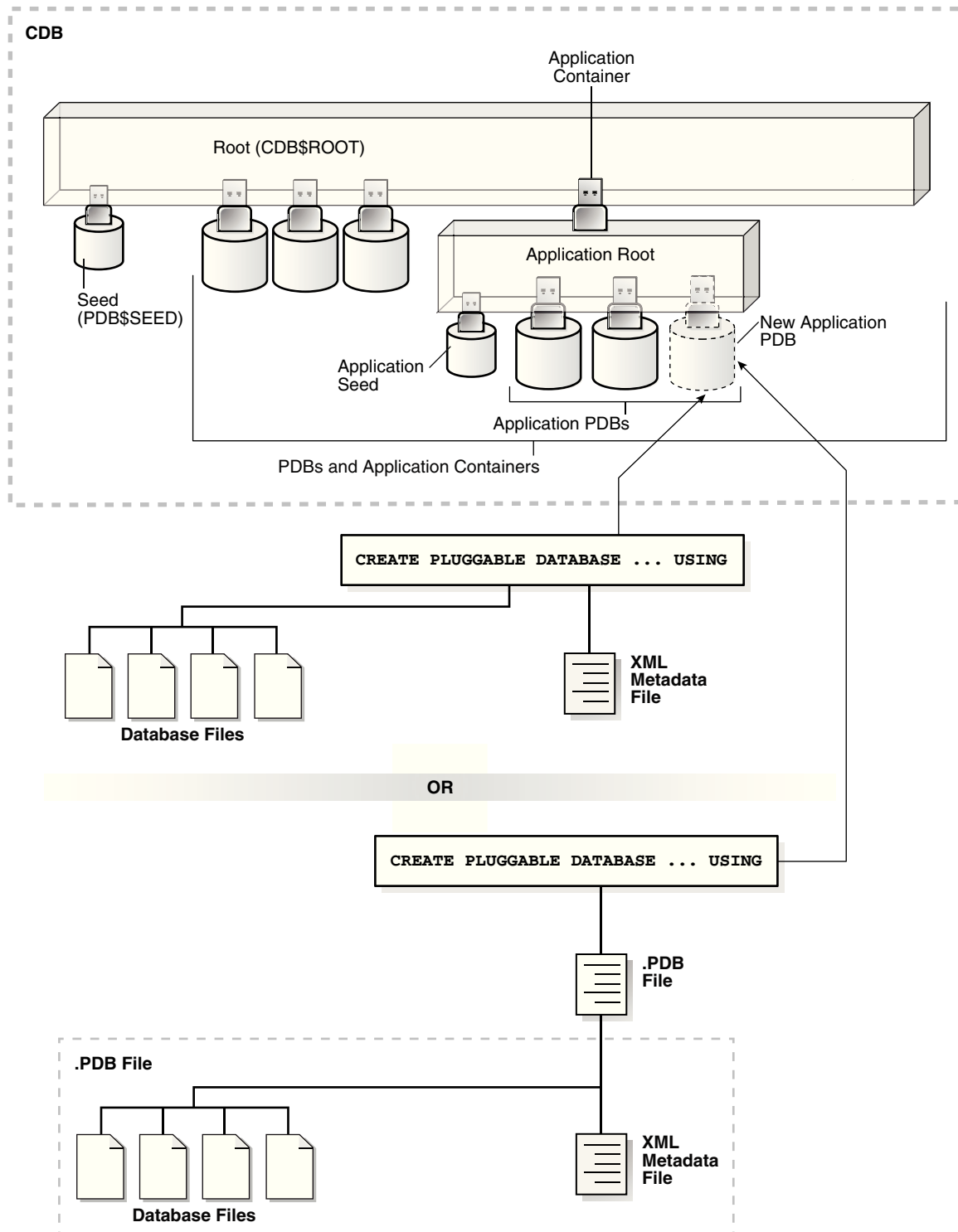
Figure 38-11 Plugging an Unplugged PDB Into an Application Root
