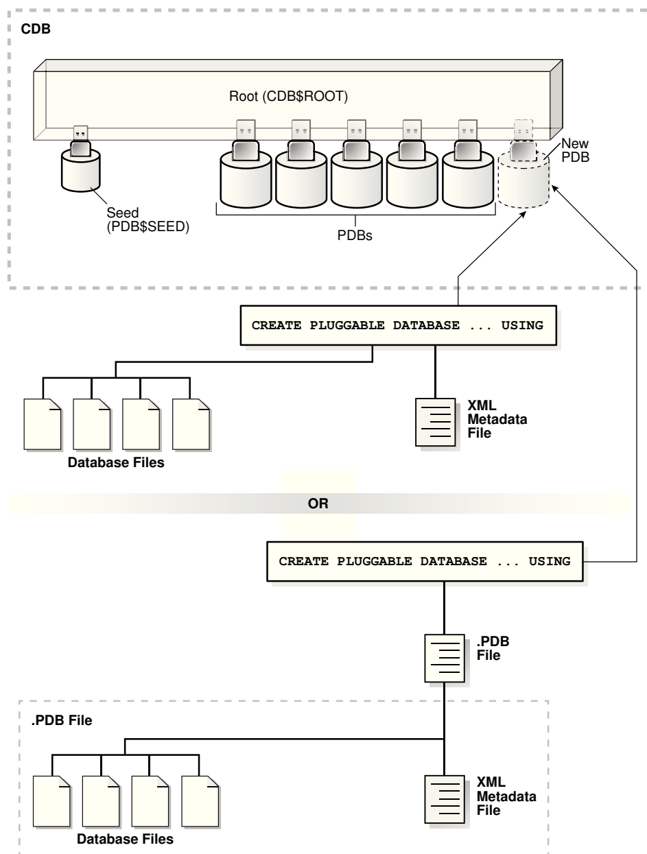
Figure 38-10 Plugging an Unplugged PDB Into a CDB Root
