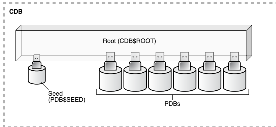
Figure 36-5 A CDB with PDBs
