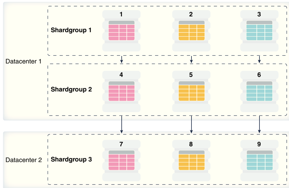
Figure 55-1 System-Managed Sharding with Data Guard Replication
