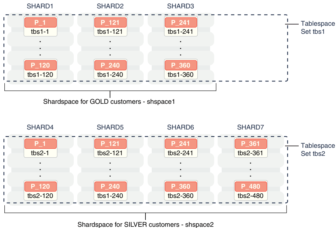
Figure 52-3 Composite Sharding
