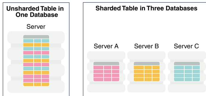
Figure 49-1 Horizontal Partitioning of a Table Across Shards
