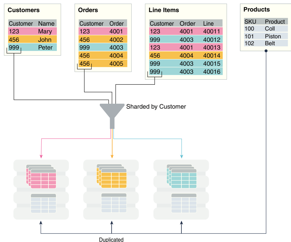
Figure 50-1 Sharded Tables and a Duplicated Table in an SDB
