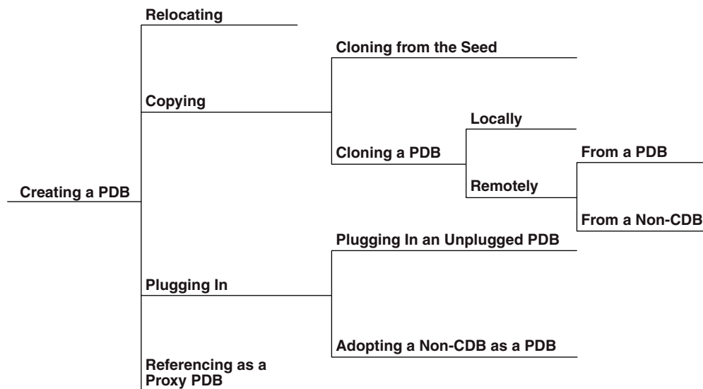
Figure 38-1 Options for Creating a PDB
