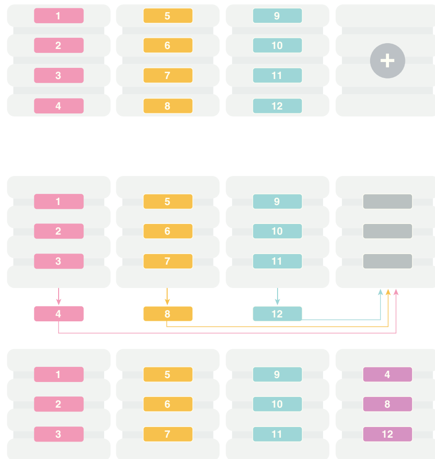
Figure 57-6 Resharding an SDB
