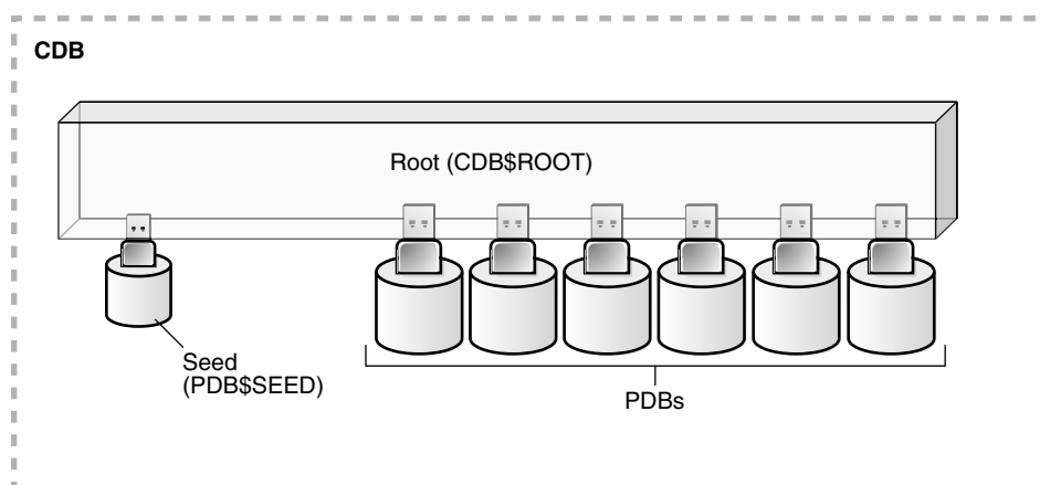
Figure 37-2 CDB with PDBs
