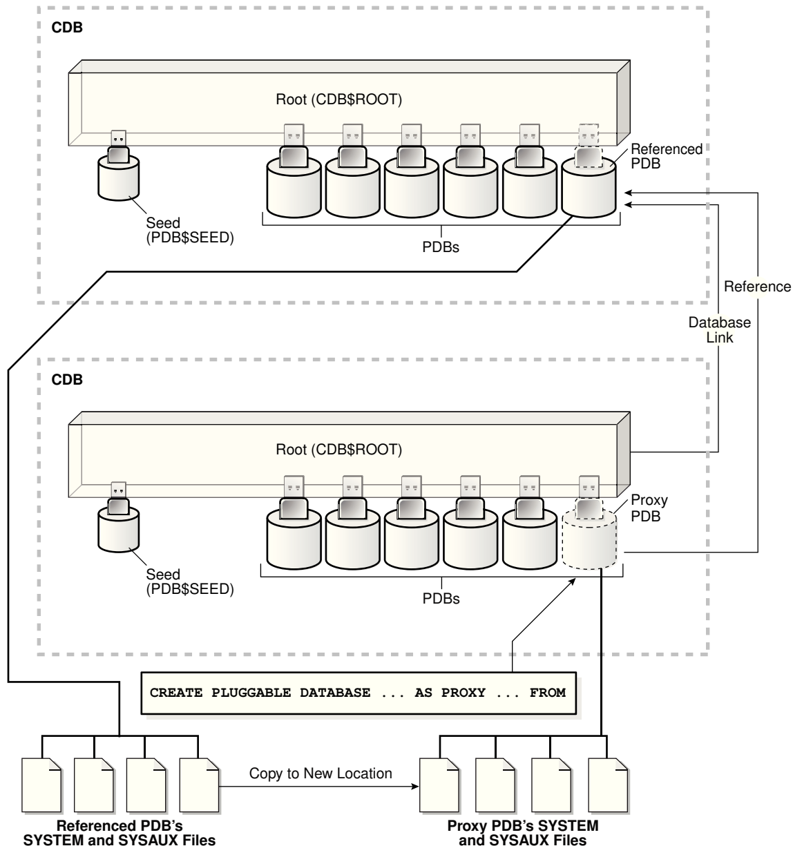
Figure 38-12 Create a Remote Proxy PDB
