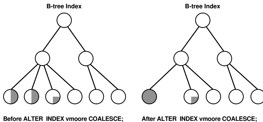
Figure 21-1 Coalescing Indexes
