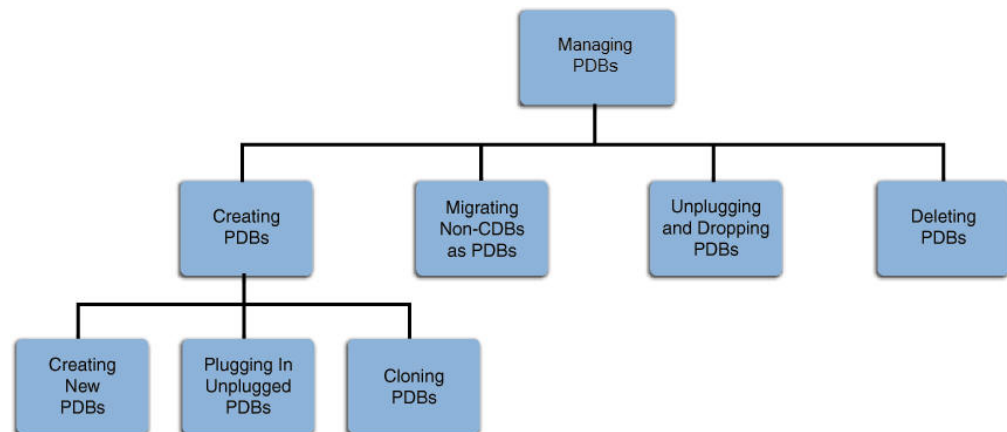
Figure 39-1 Managing PDBs
