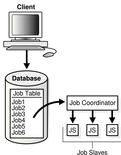
Figure 28-6 Scheduler Components
