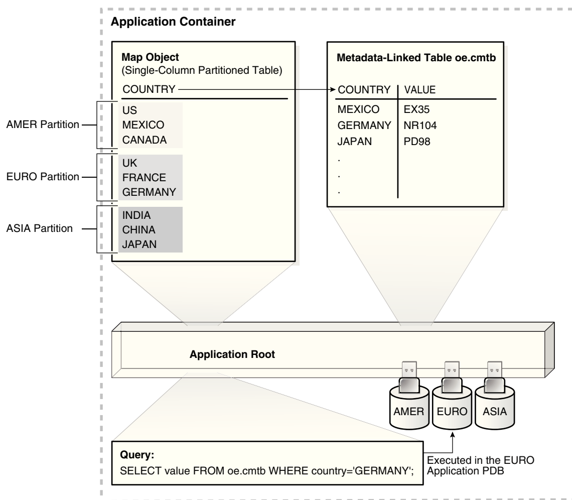
Figure 44-3 Container Map
