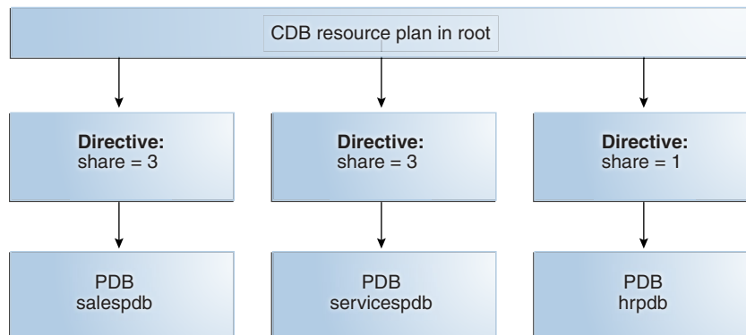
Figure 46-1 Shares in a CDB Resource Plan
