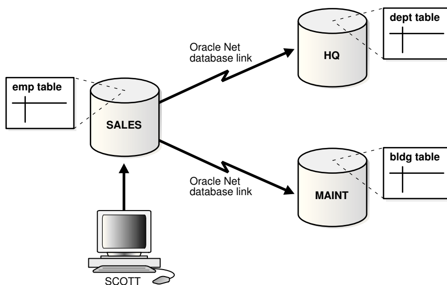
Figure 34-1 Distributed System
