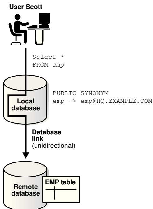
Figure 31-3 Database Link
