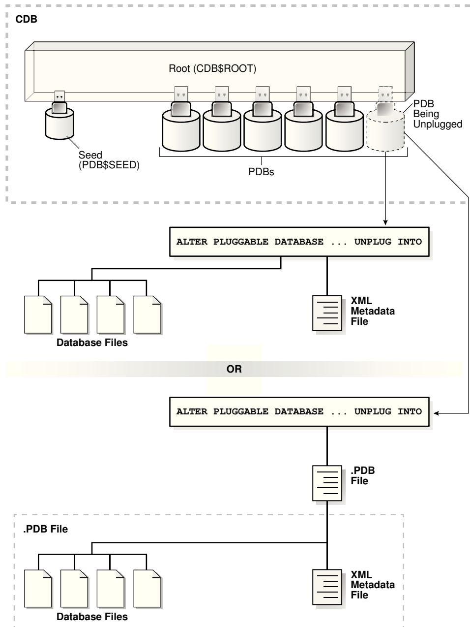
Figure 38-15 Unplug a PDB
