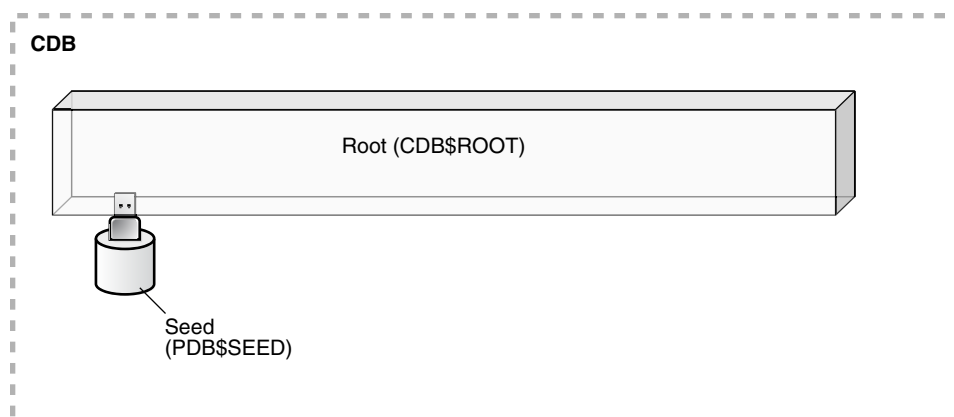
Figure 37-1 A Newly Created CDB
