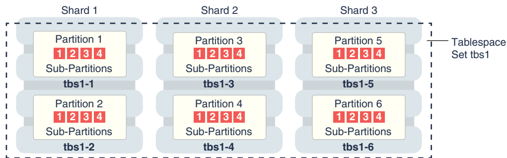
Figure 52-4 Subpartitions Stored in the Tablespace of the Parent Partition
