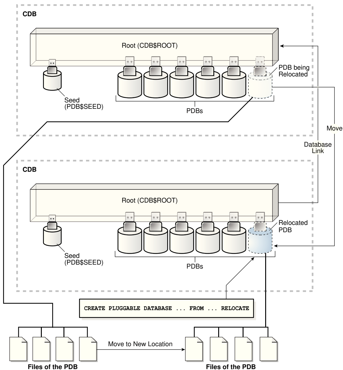
Figure 38-8 Relocate a PDB
