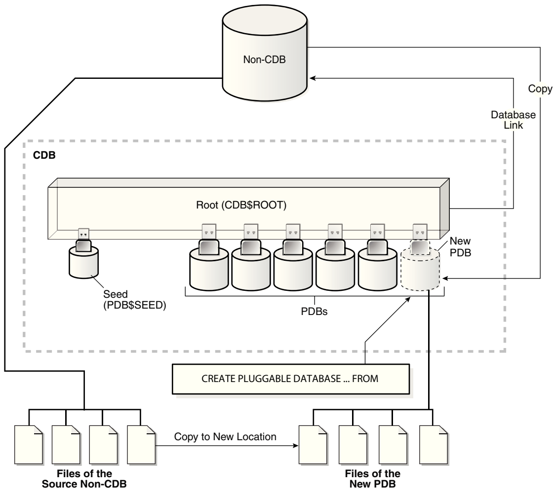
Figure 38-6 Creating a PDB by Cloning a Non-CDB
