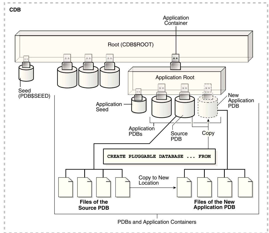
Figure 38-7 Clone a PDB in an Application Container
