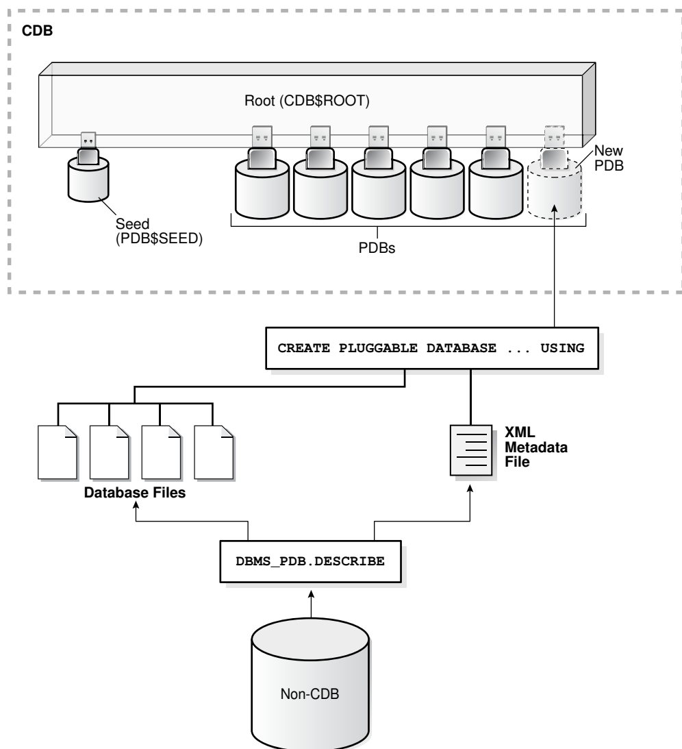
Figure 38-14 Plug In a Non-CDB Using the DBMS_PDB.DESCRIBE Procedure
