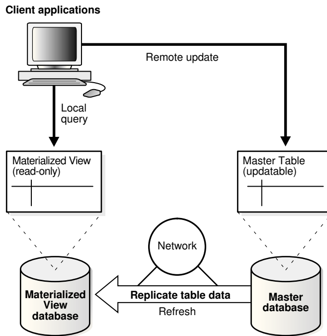
Figure 58-1 Read-Only Materialized View
