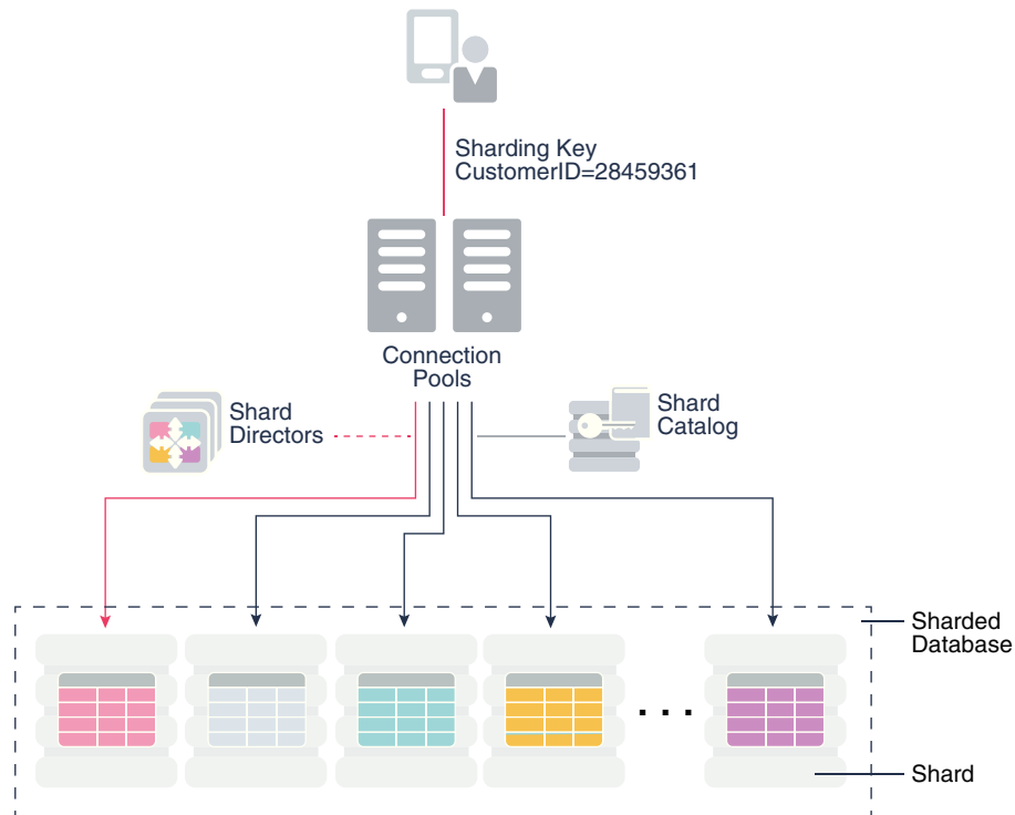
Figure 49-2 Oracle Sharding Architecture
