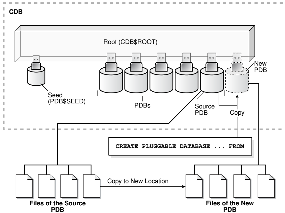
Figure 38-4 Clone a Local PDB
