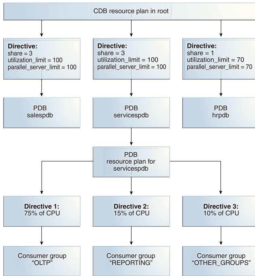
Figure 46-4 A CDB Resource Plan and a PDB Resource Plan
