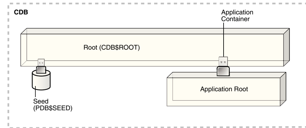
Figure 36-4 An Application Container
