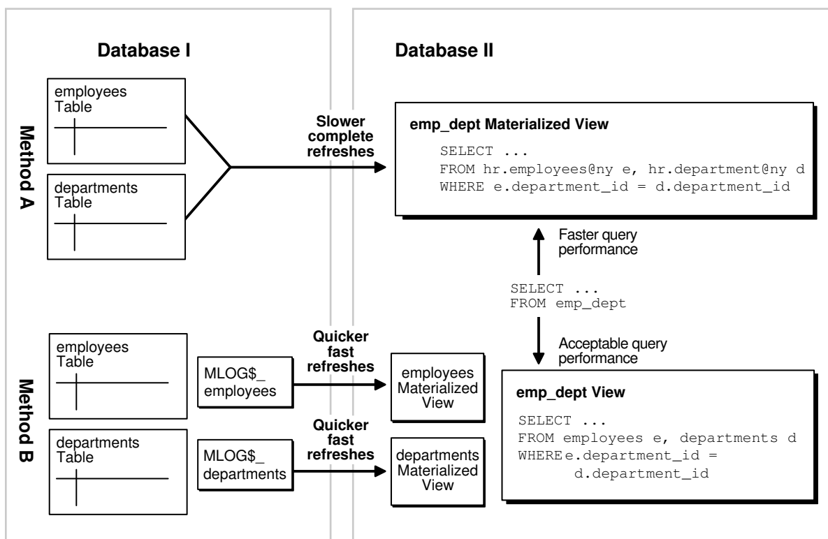
Figure 58-2 Comparison of Simple and Complex Materialized Views
