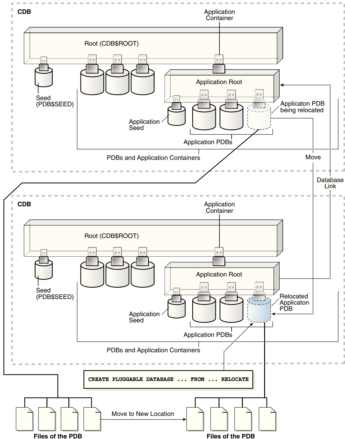
Figure 38-9 Relocate a PDB Into an Application Container
