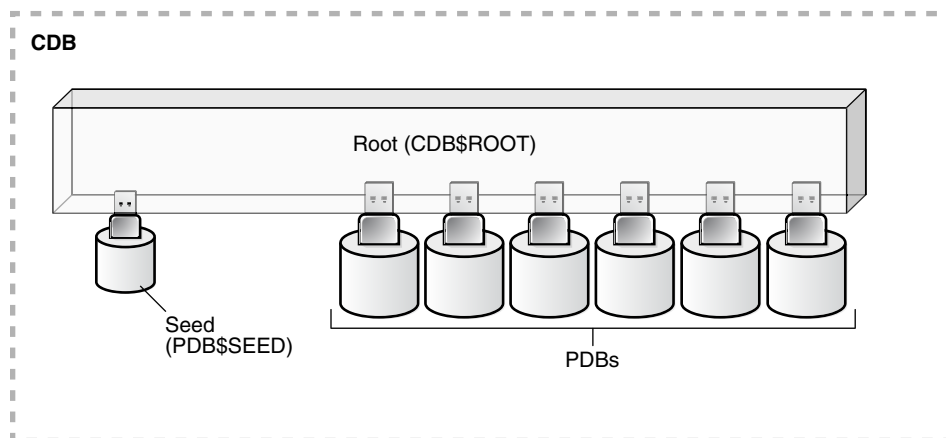
Figure 36-1 CDB with PDBs
