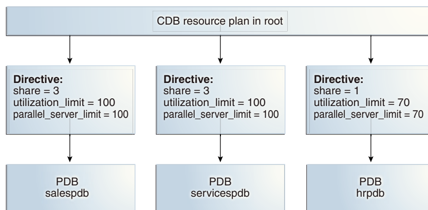
Figure 46-2 Shares and Utilization Limits in a CDB Resource Plan
