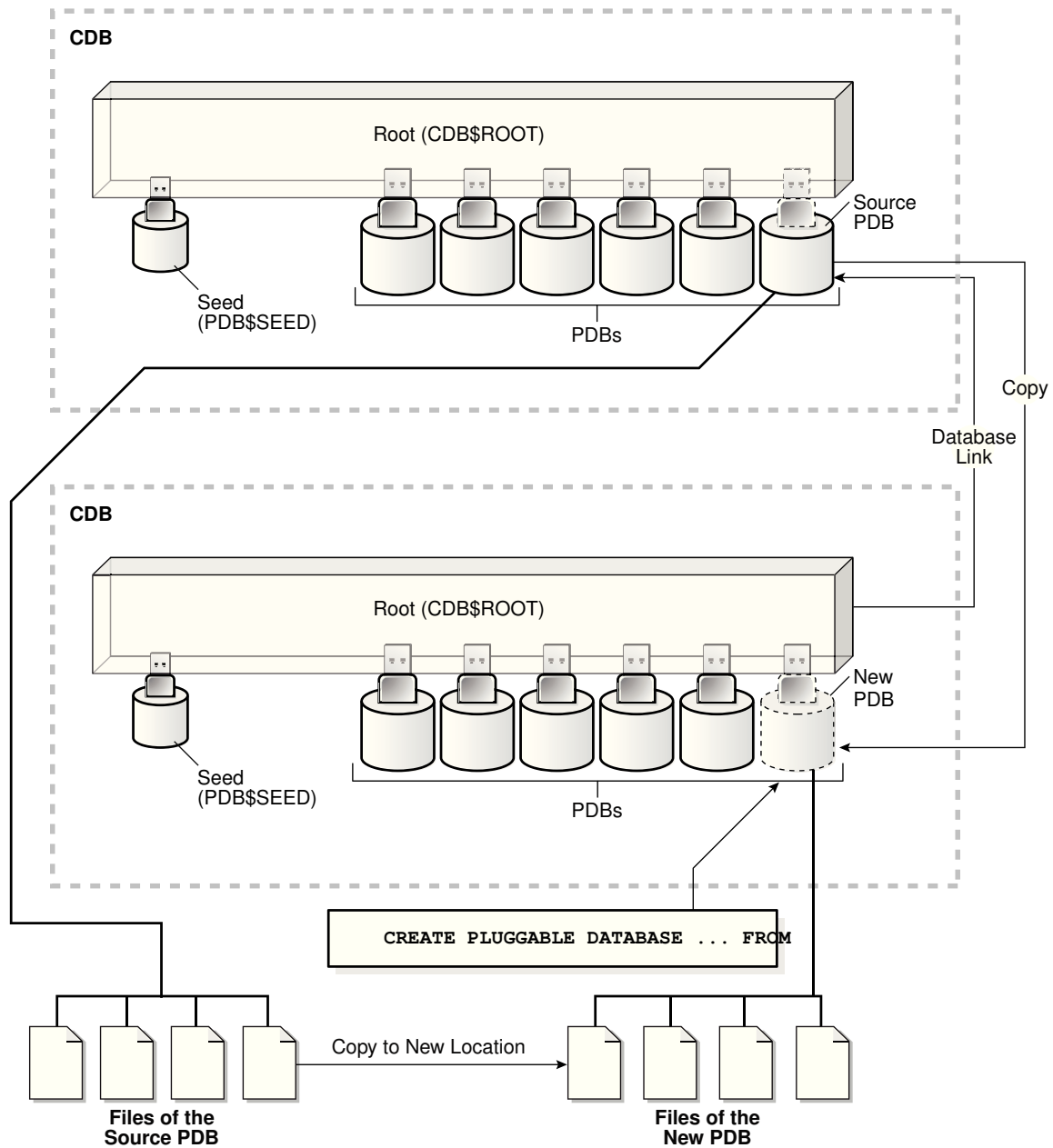
Figure 38-5 Creating a PDB by Cloning a Remote PDB
