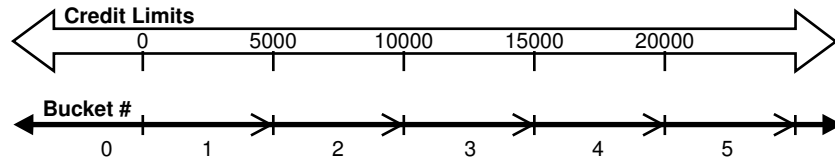
Figure 19-4 Bucket Assignments
