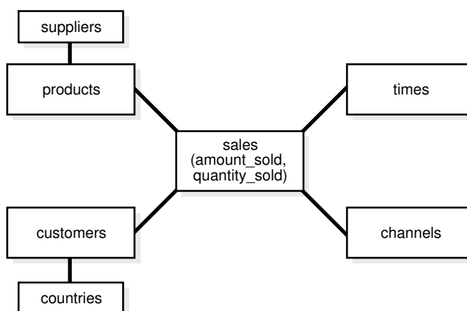
Figure 2-3 Snowflake Schema
