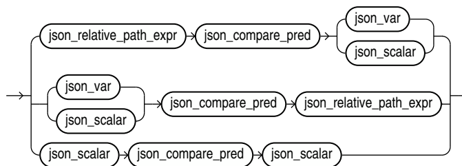
Figure C-13 json_comparison
