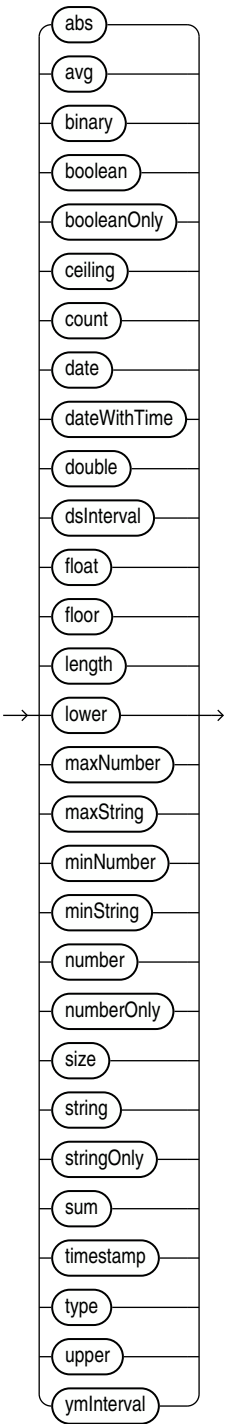
Figure C-9 json_item_method
