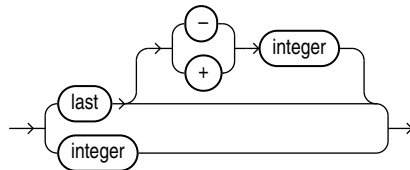
Figure C-7 json_array_index
