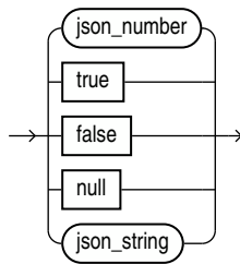
Figure C-17 json_scalar
