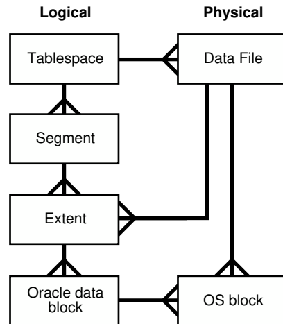
Figure 15-1 Logical and Physical Storage
