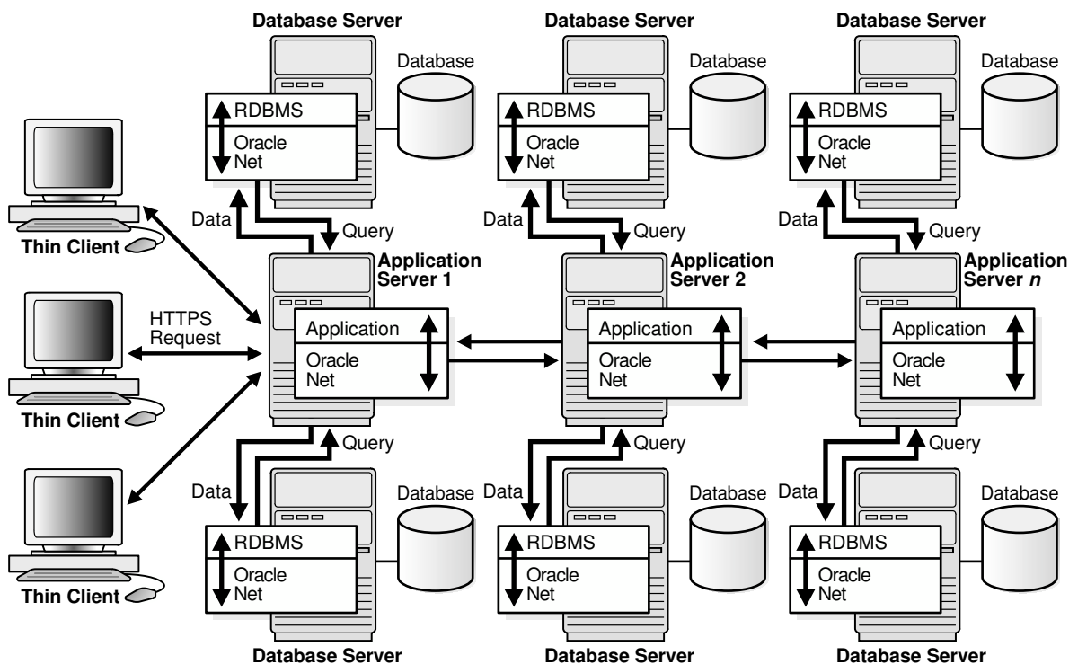
Figure 19-3 A Multitier Architecture Environment
