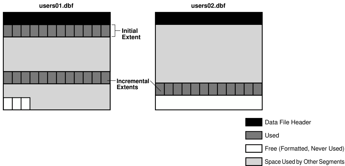
Figure 15-18 Incremental Extent of a Segment
