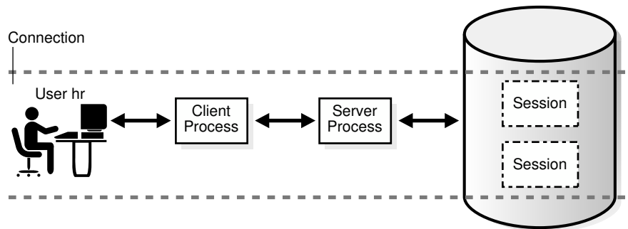
Figure 18-3 Two Sessions in One Connection
