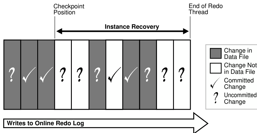
Figure 16-5 Checkpoint Position in Online Redo Log
