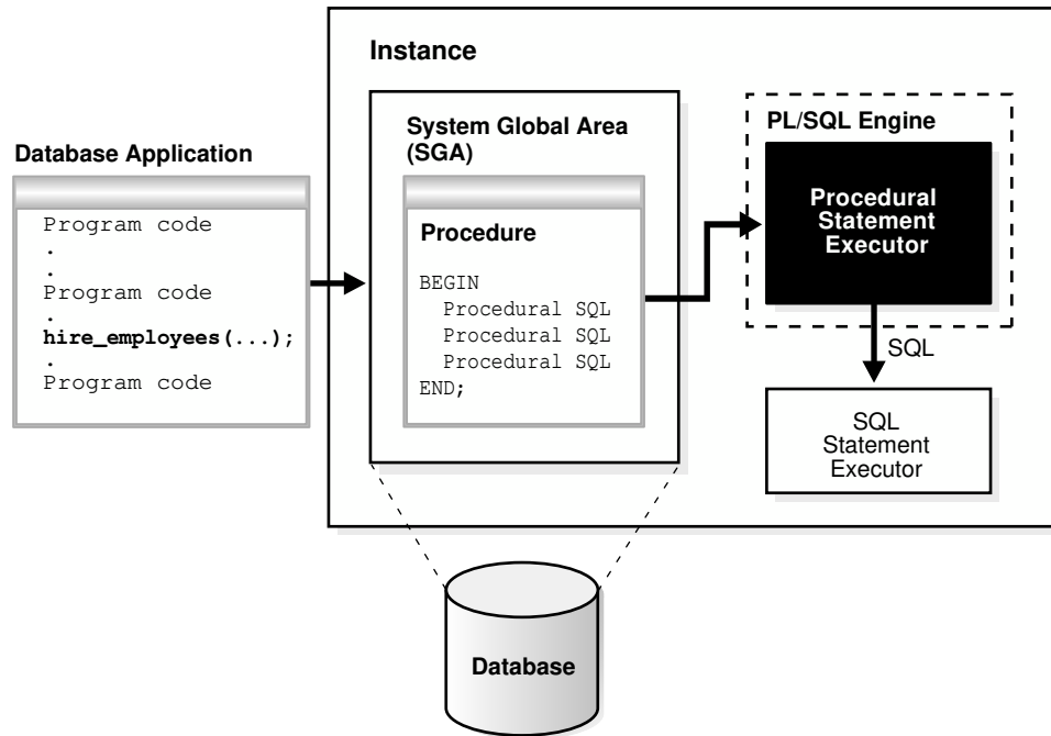
Figure 11-3 The PL/SQL Engine and Oracle Database
