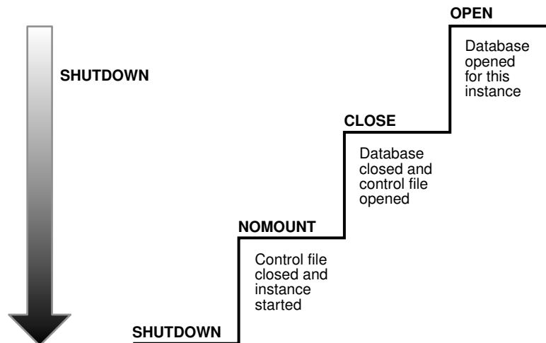
Figure 16-4 Instance and Database Shutdown Sequence
