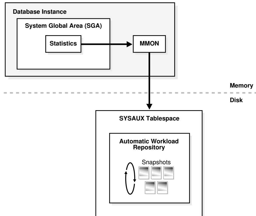
Figure 22-9 Automatic Workload Repository (AWR)
