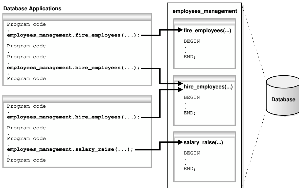
Figure 11-2 Calling Subprograms in a PL/SQL Package
