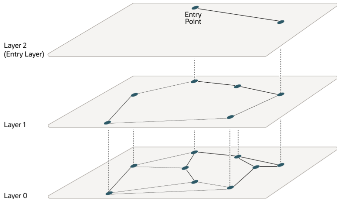
Figure 21-4 Hierarchical Navigable Small World Graphs
