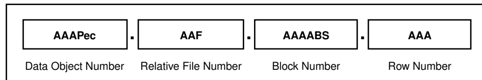
Figure 15-9 ROWID Format
