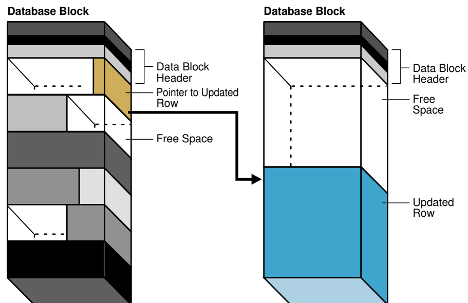
Figure 15-14 Row Migration
