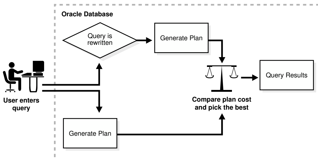
Figure 6-10 Query Rewrite
