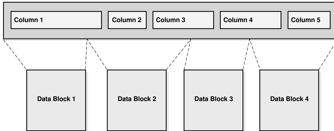
Figure 4-7 Compression Unit
