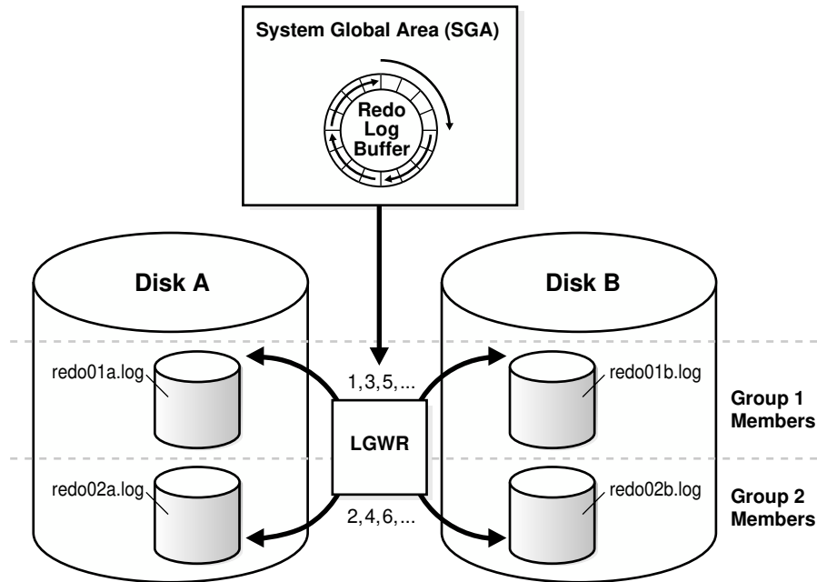
Figure 14-8 Multiple Copies of Online Redo Log Files
