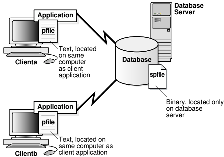
Figure 16-7 Multiple Initialization Parameter Files
