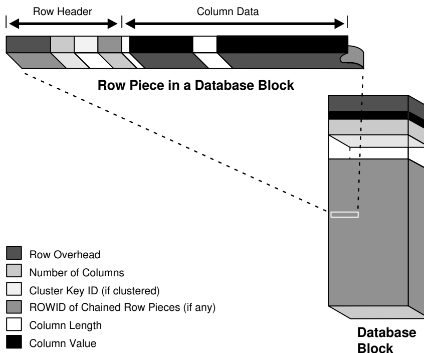
Figure 15-8 The Format of a Row Piece
