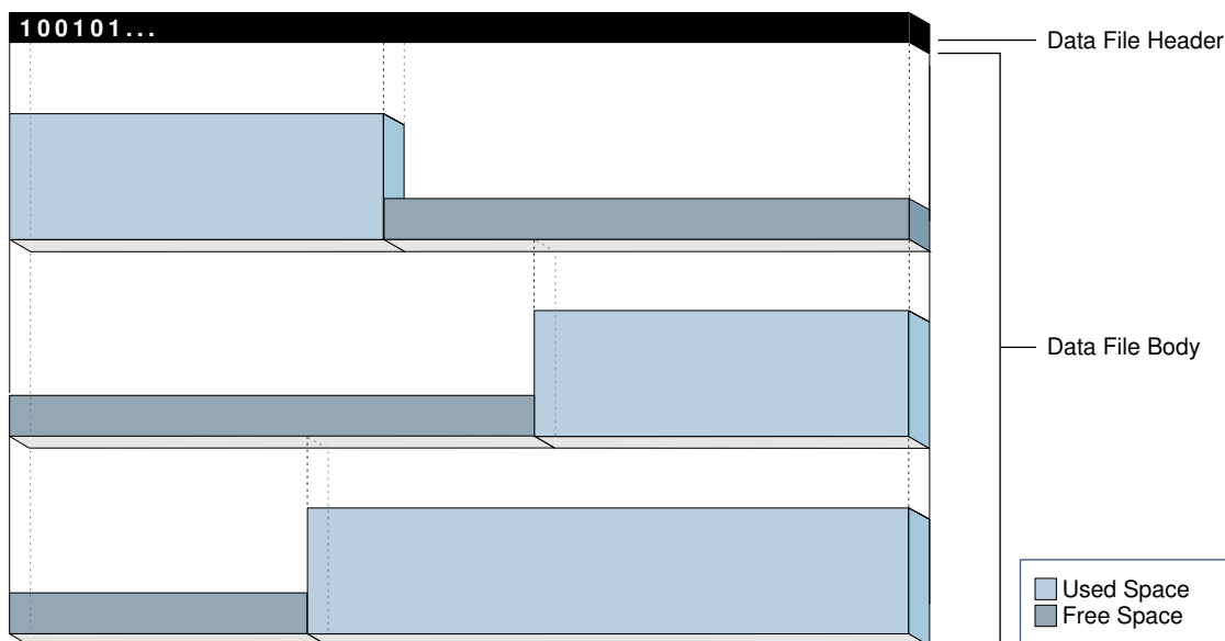
Figure 15-4 Bitmap-Managed Storage
