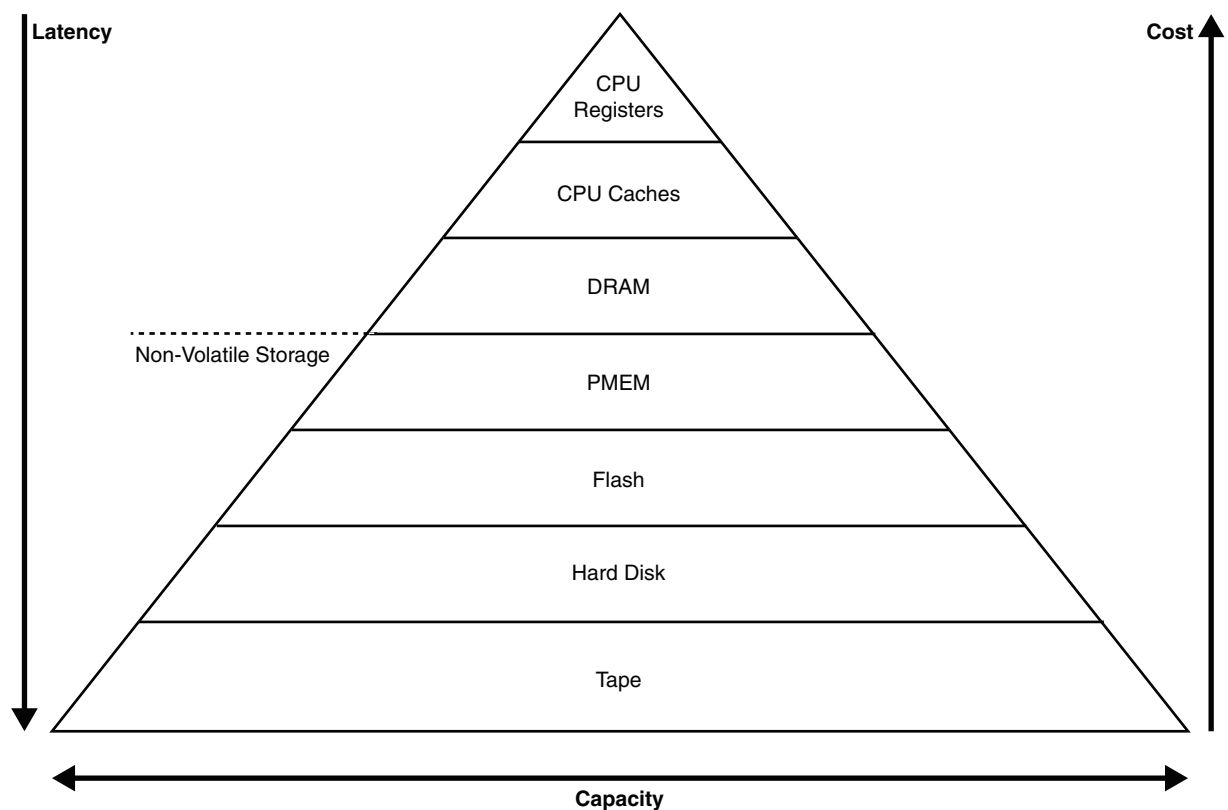
Figure 14-4 Storage Pyramid
