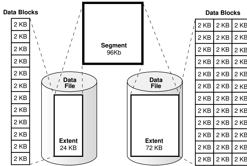
Figure 15-2 Segments, Extents, and Data Blocks Within a Tablespace
