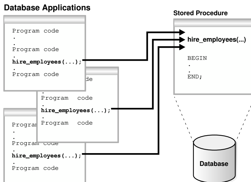
Figure 11-1 Multiple Executions of a Stored Procedure
