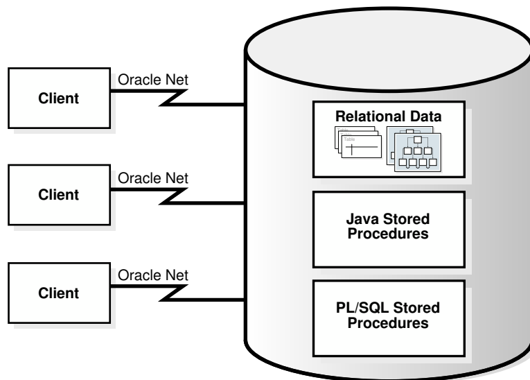
Figure 11-4 Two-Tier Client/Server Configuration
