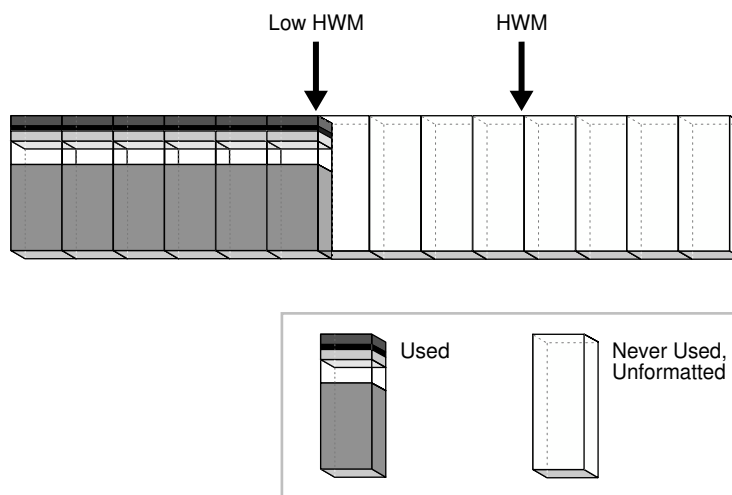
Figure 15-25 HWM and Low HWM
