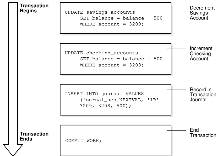
Figure 13-1 A Banking Transaction
