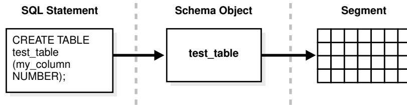
Figure 15-19 Creation of a User Segment
