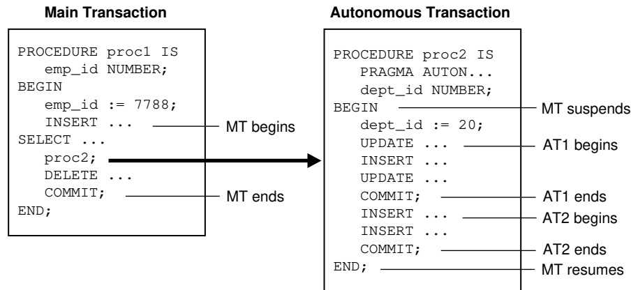
Figure 13-4 Transaction Control Flow
