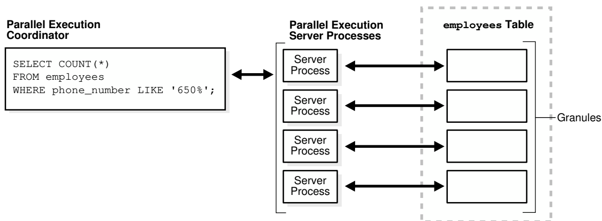
Figure 18-7 Parallel Full Table Scan
