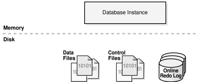
Figure 14-1 Database Instance and Database Files
