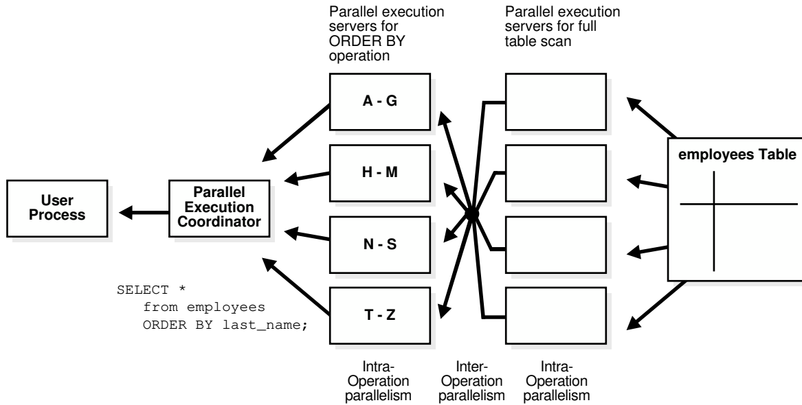
Figure 18-6 Producers and Consumers
