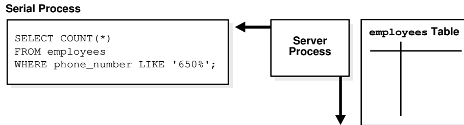
Figure 18-5 Serial Full Table Scan
