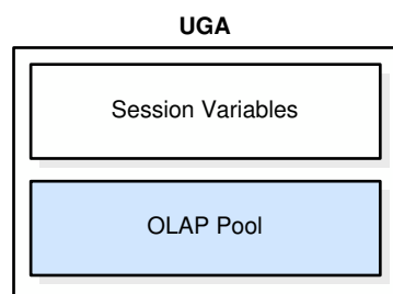
Figure 17-13 User Global Area (UGA)
