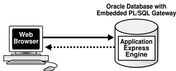
Figure 23-1 Application Express with Embedded PL/SQL Gateway
