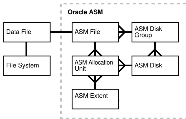
Figure 14-2 Oracle ASM Components
