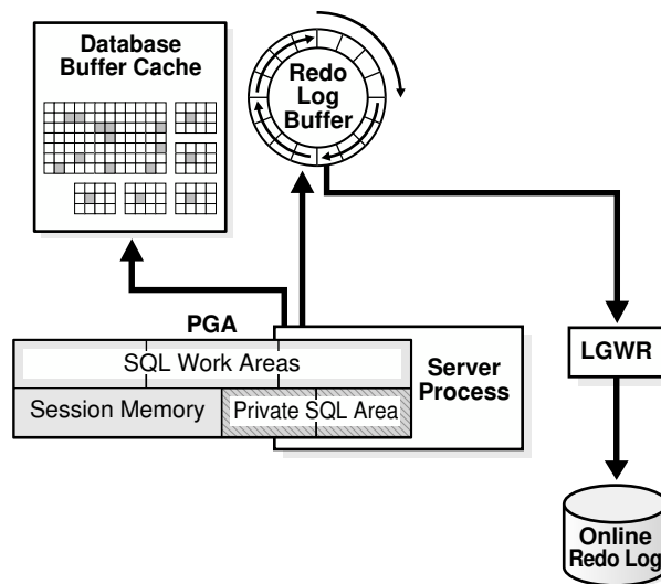
Figure 17-4 Redo Log Buffer
