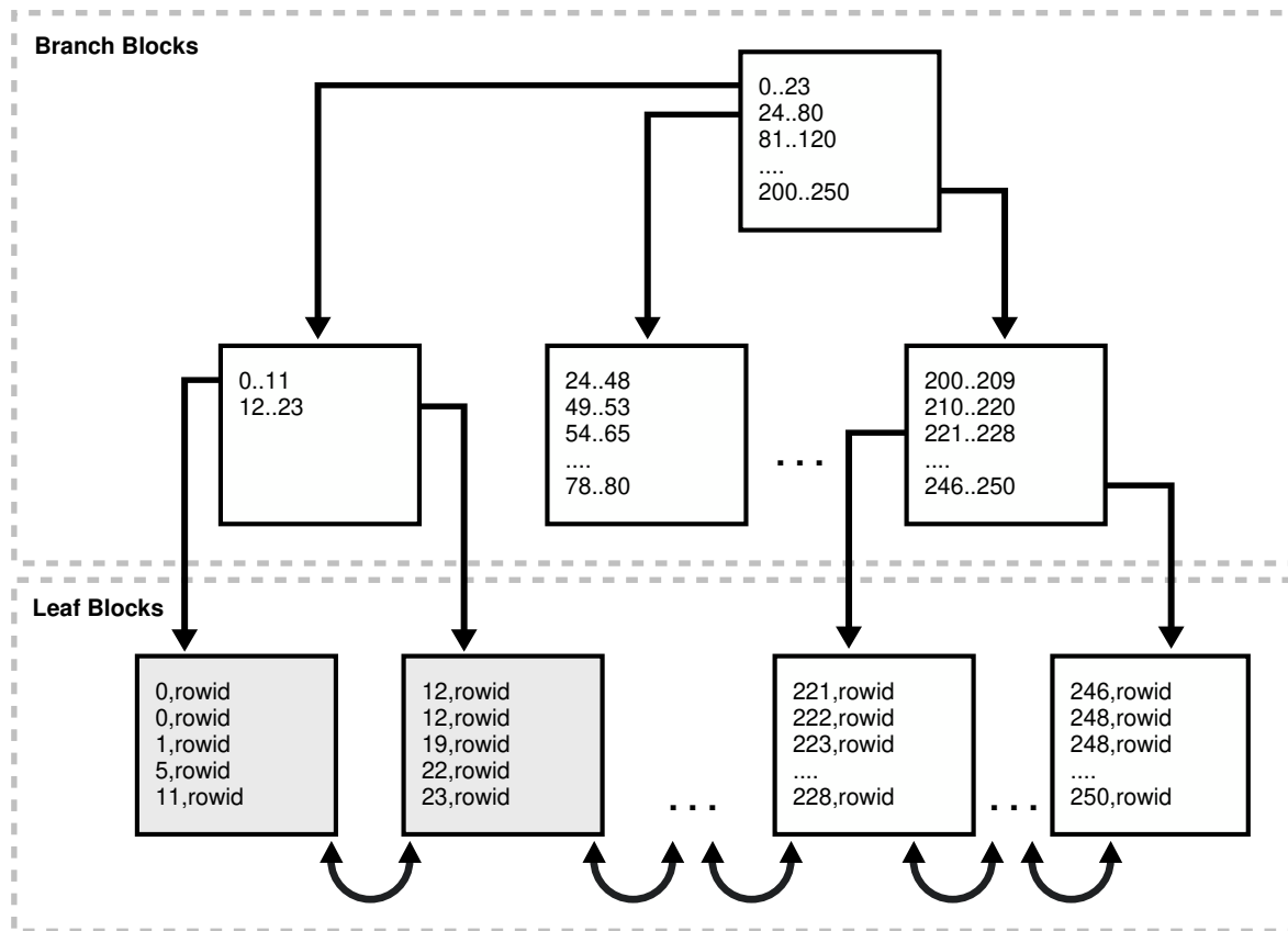
Figure 15-16 Index After Coalescing
