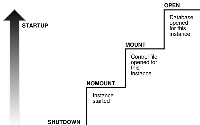
Figure 16-3 Instance and Database Startup Sequence
