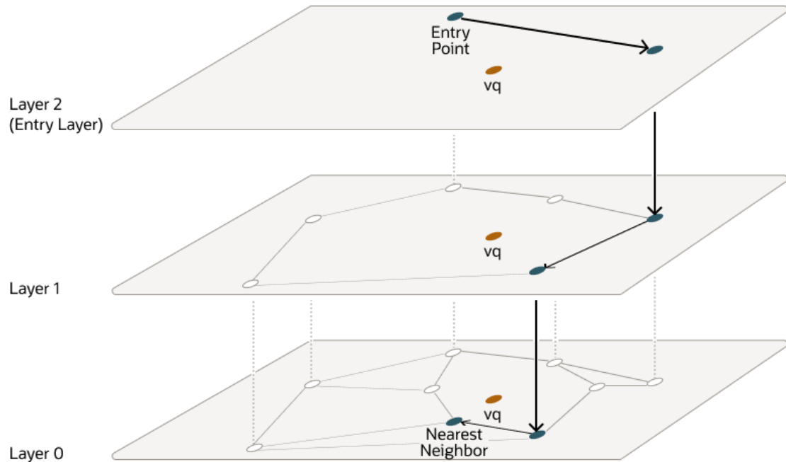
Figure 21-5 Hierarchical Navigable Small World Graphs Search
