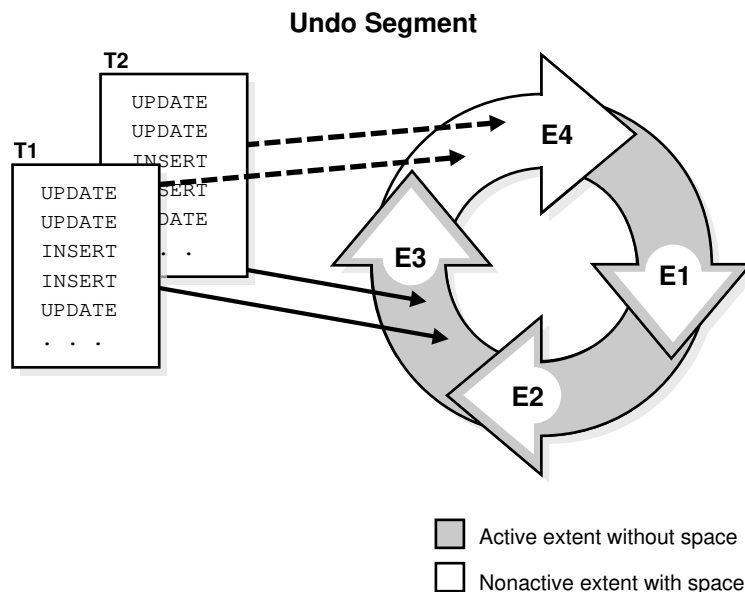
Figure 15-21 Ring of Allocated Extents in an Undo Segment
