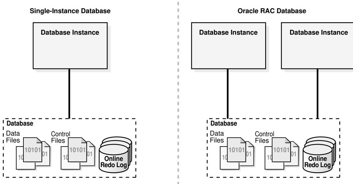
Figure 16-2 Database Instance Configurations
