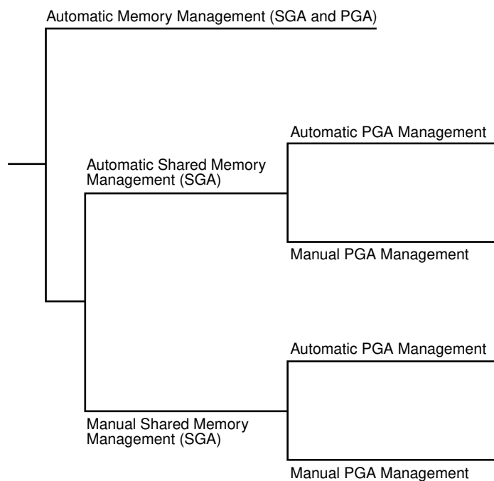
Figure 22-5 Memory Management Methods
