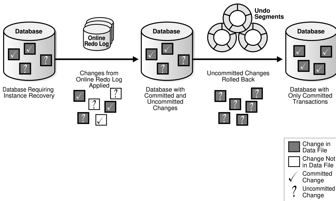
Figure 16-6 Basic Instance Recovery Steps: Rolling Forward and Rolling Back
