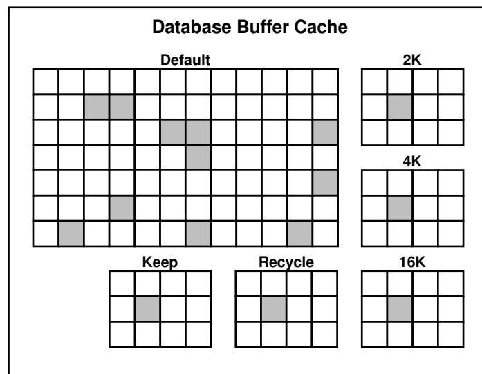
Figure 17-3 Database Buffer Cache
