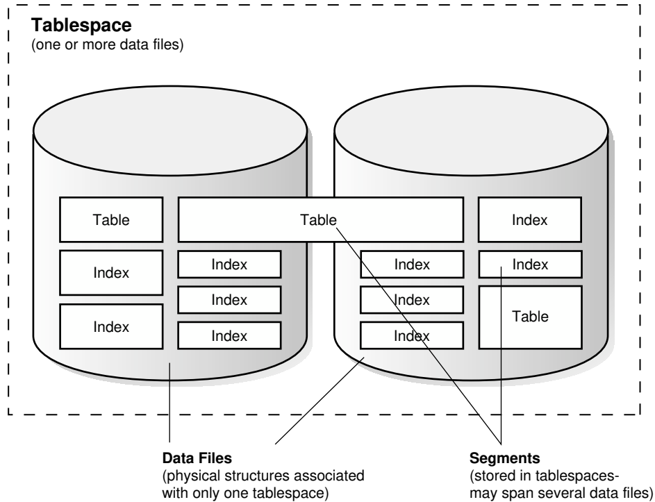
Figure 14-5 Data Files and Tablespaces
