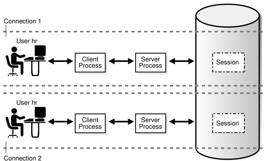
Figure 18-2 One Session for Each Connection
