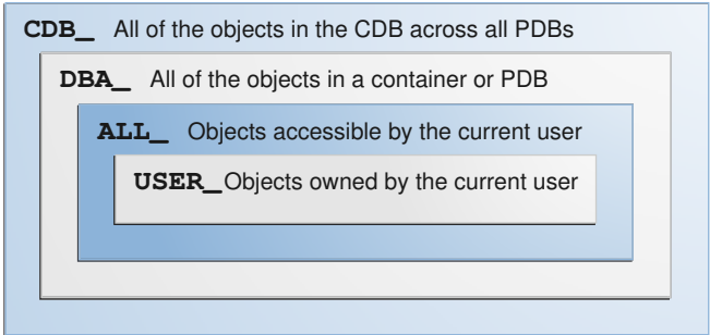
Figure 9-3 Dictionary Views in a CDB
