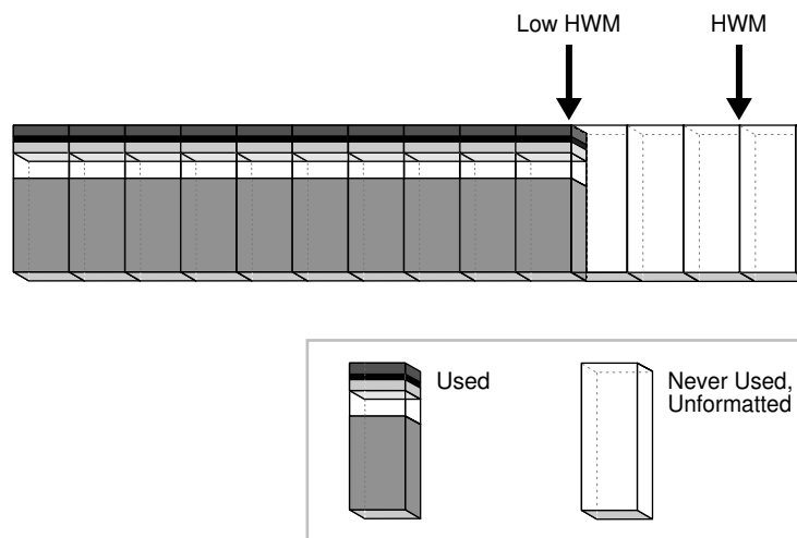
Figure 15-27 Advancing HWM and Low HWM
