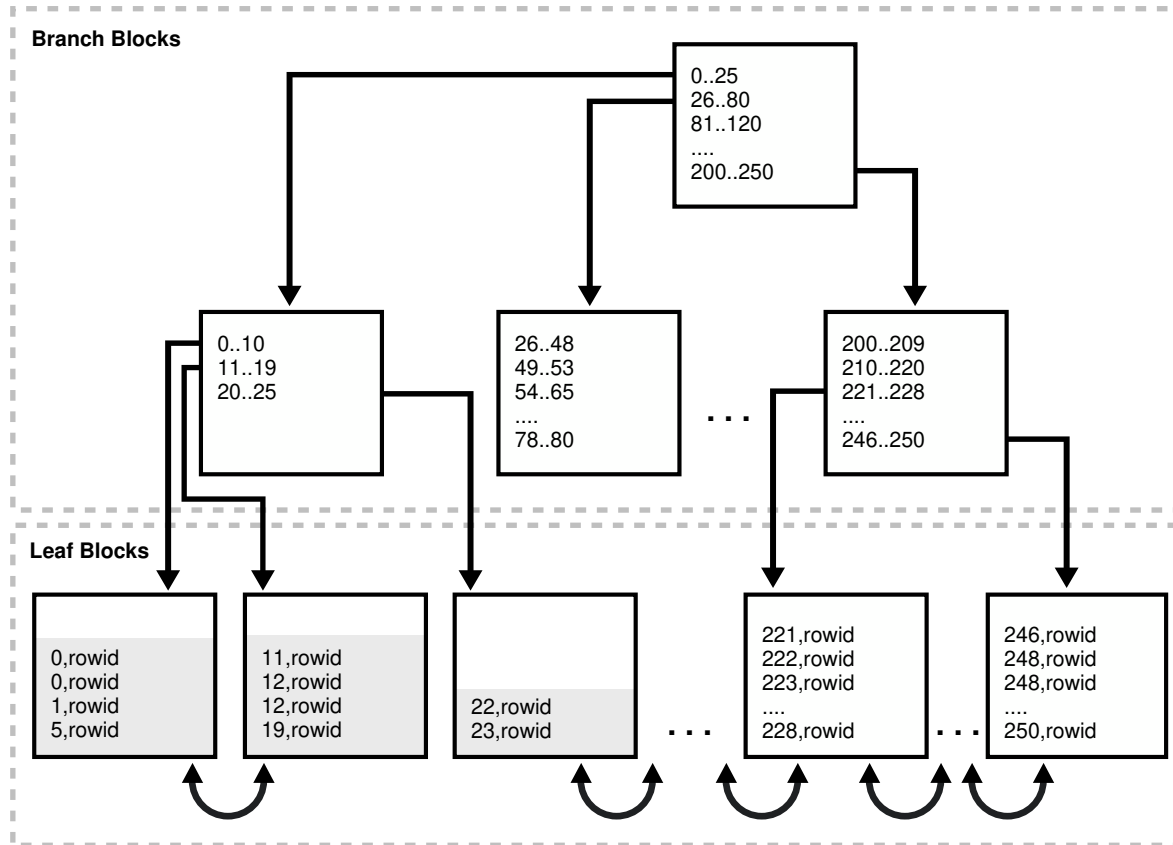
Figure 15-15 Index Before Coalescing
