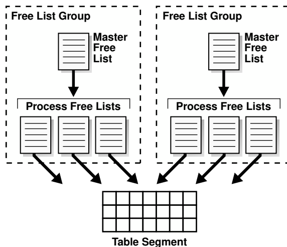
Figure 15-5 Free List Groups
