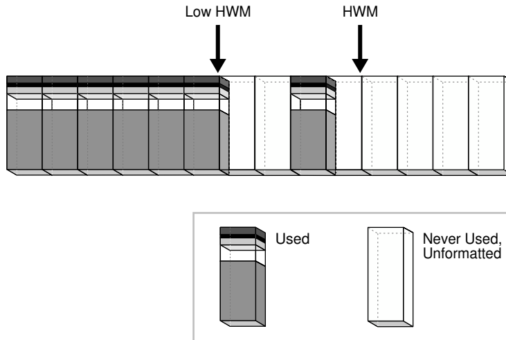
Figure 15-26 HWM and Low HWM
