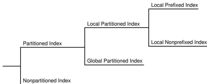
Figure 6-2 Index Partitioning Options
