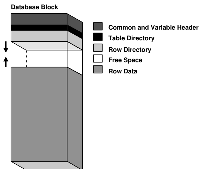
Figure 15-7 Data Block Format
