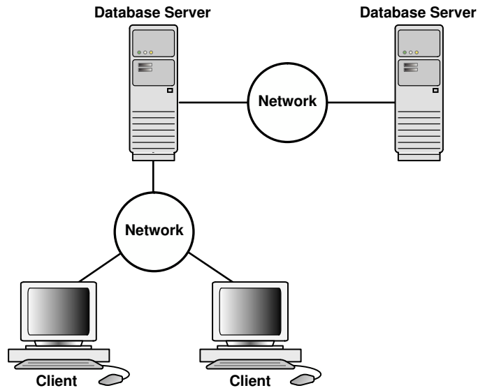
Figure 19-2 Client/Server Architecture and Distributed Database
