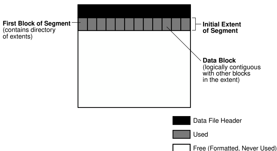
Figure 15-17 Initial Extent of a Segment
