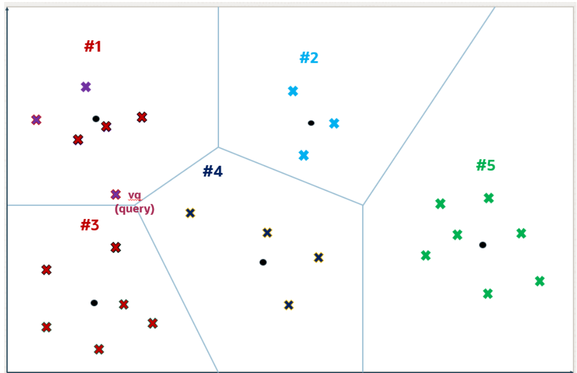
Figure 21-8 Inverted File Flat Index
