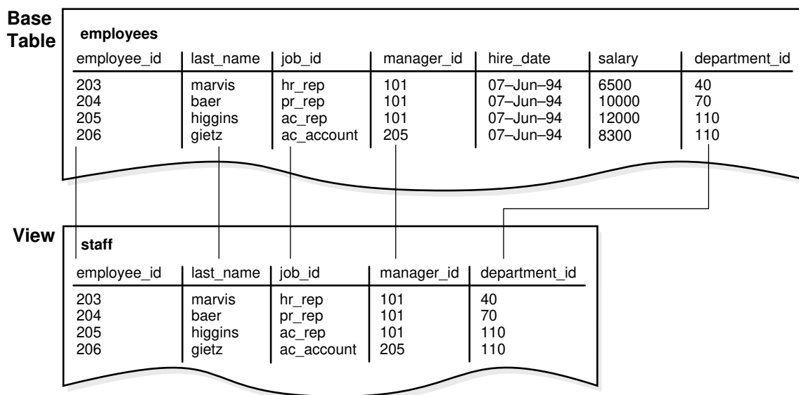
Figure 6-8 View
