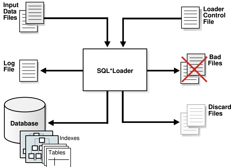
Figure 22-1 SQL*Loader Session
