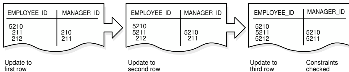
Figure 7-5 Constraint Checking
