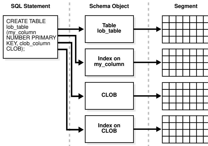
Figure 15-20 Multiple Segments
