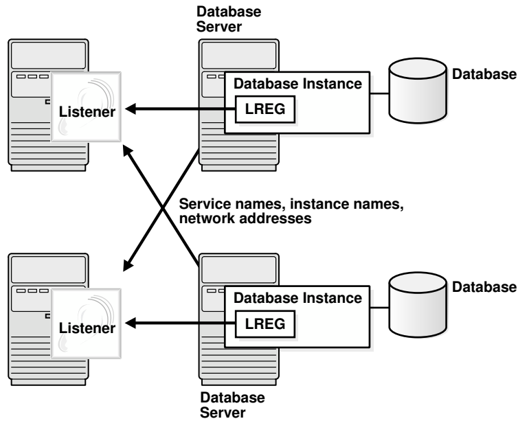
Figure 19-4 Two Listeners
