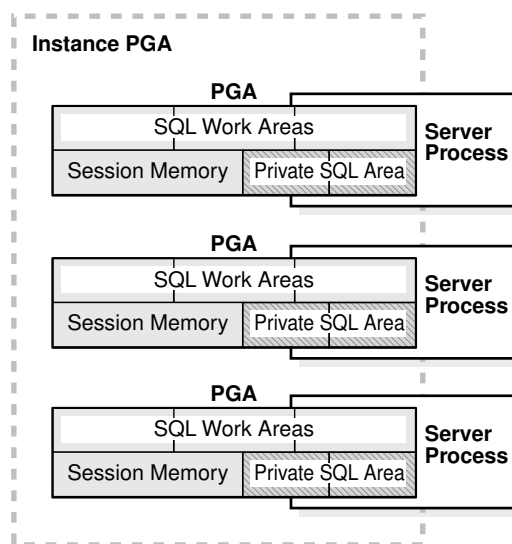
Figure 17-10 Instance PGA
