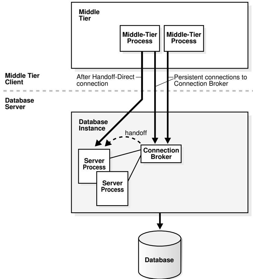
Figure 19-10 DRCP
