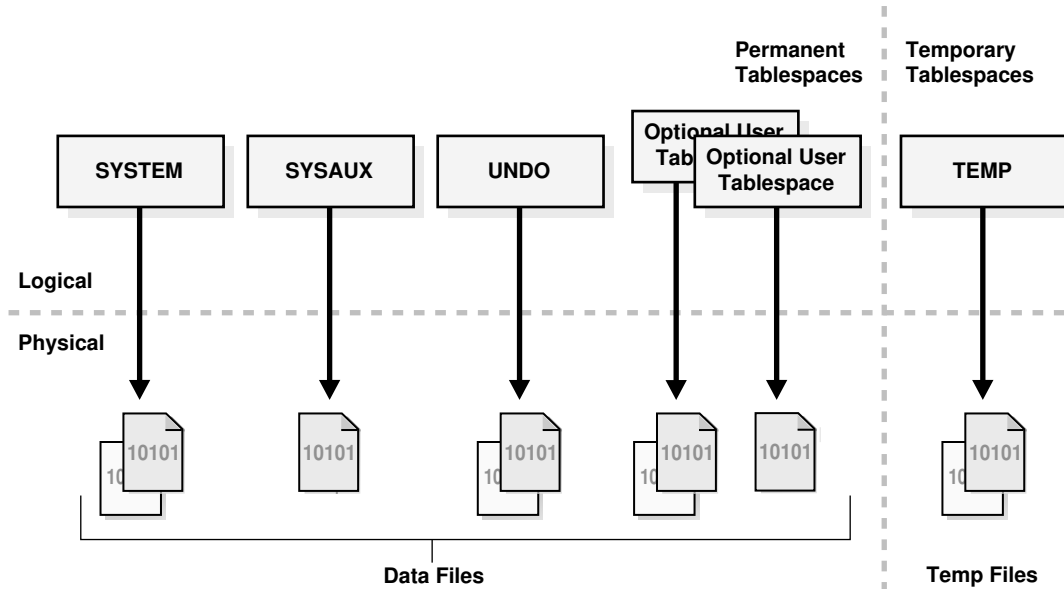
Figure 15-28 Tablespaces
