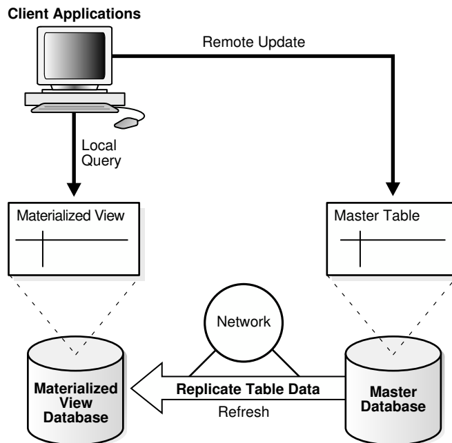
Figure 6-9 Materialized View
