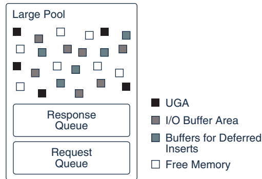
Figure 17-7 Large Pool
