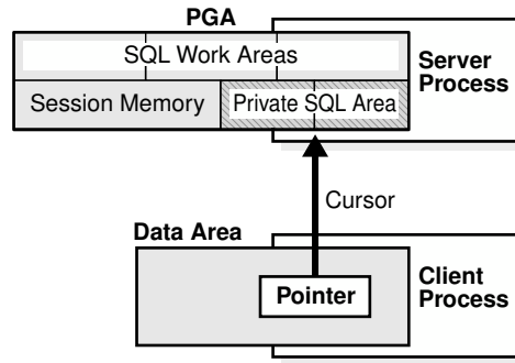
Figure 17-12 Cursor
