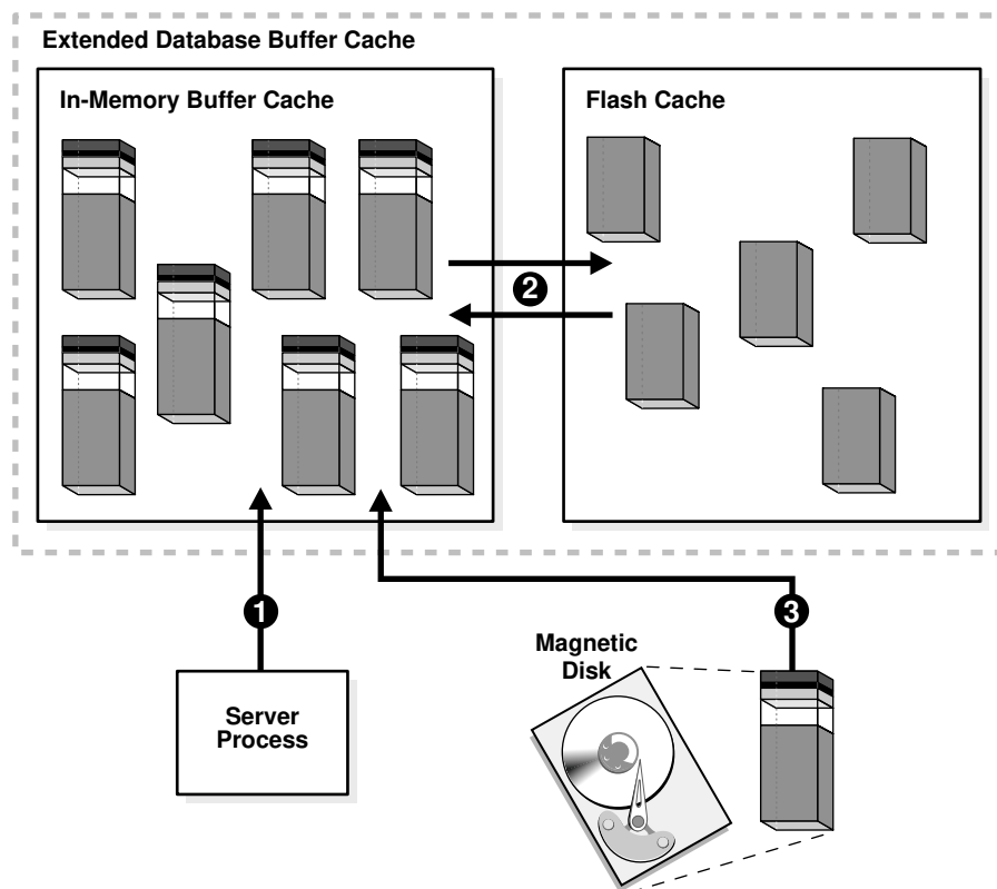
Figure 17-2 Buffer Search
