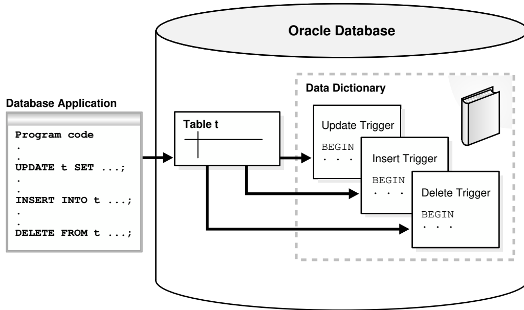
Figure 11-7 Triggers
