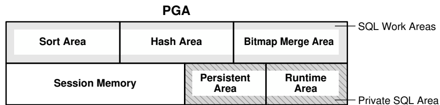
Figure 17-11 PGA Contents
