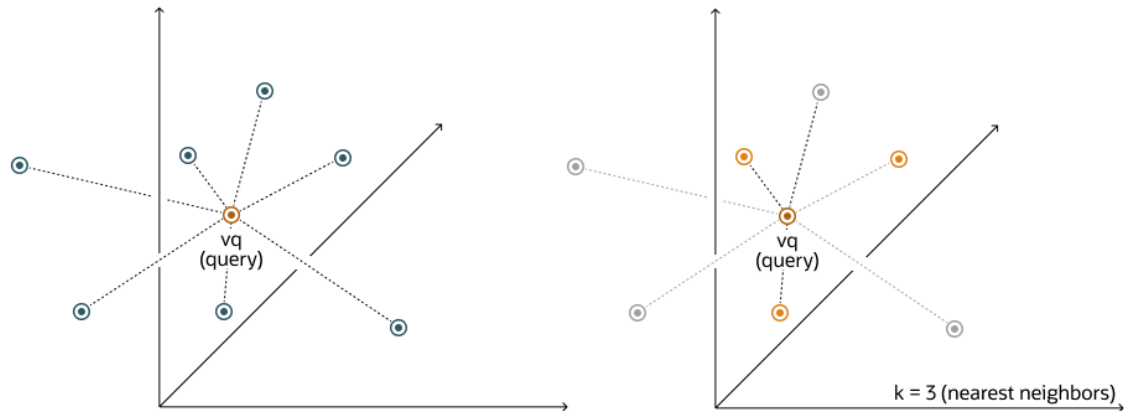
Figure 21-13 Exact Search
