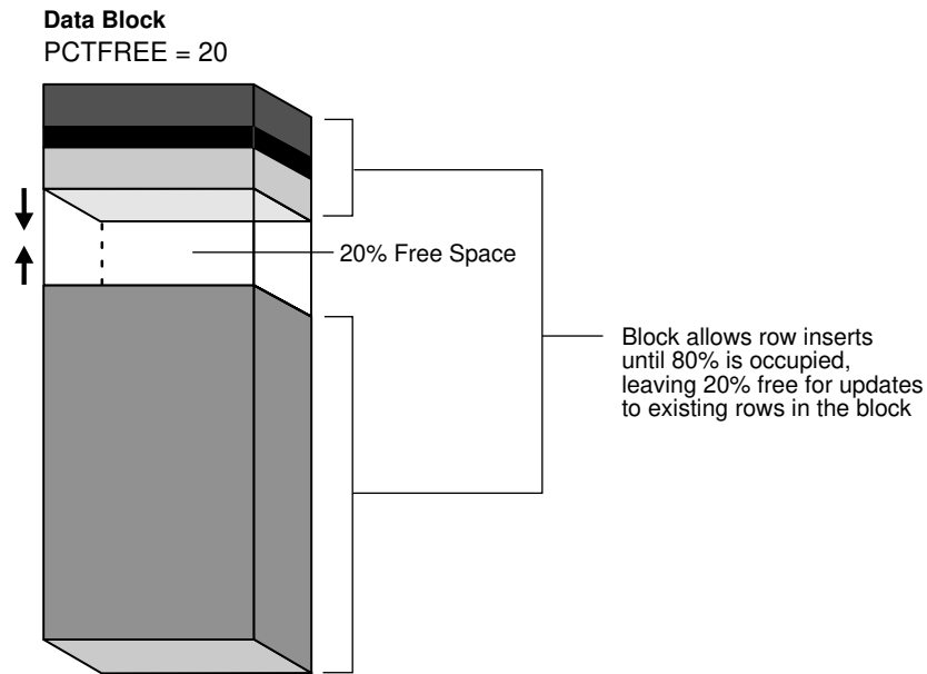
Figure 15-10 PCTFREE
