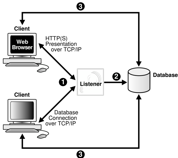
Figure 19-5 Listener Architecture
