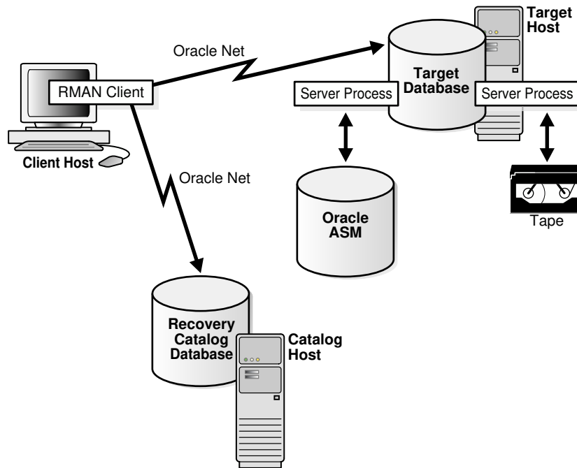
Figure 22-3 RMAN Architecture
