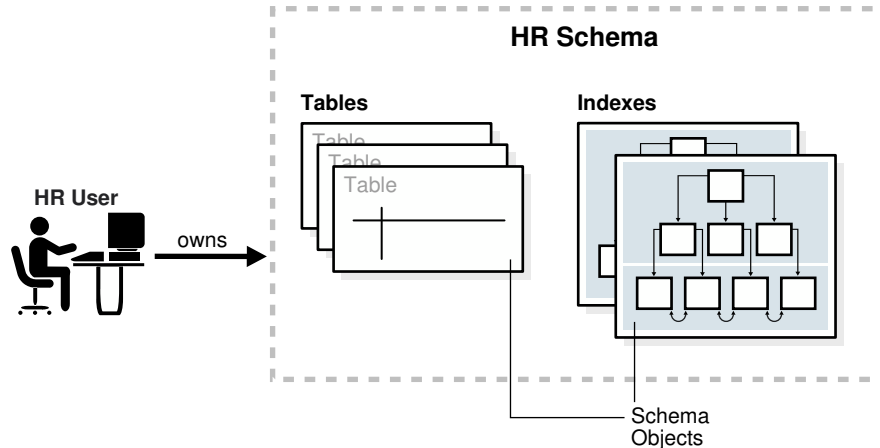
Figure 4-1 HR Schema
