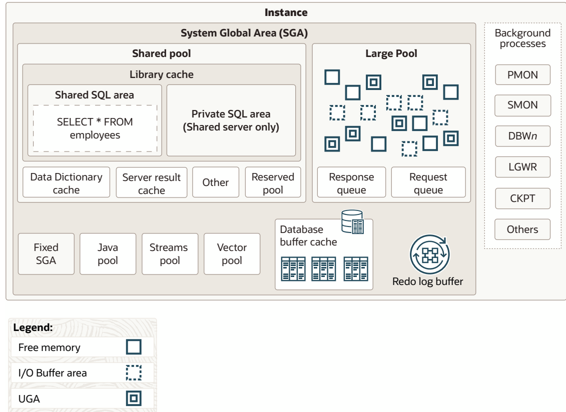
Figure 16-1 Database Instance
