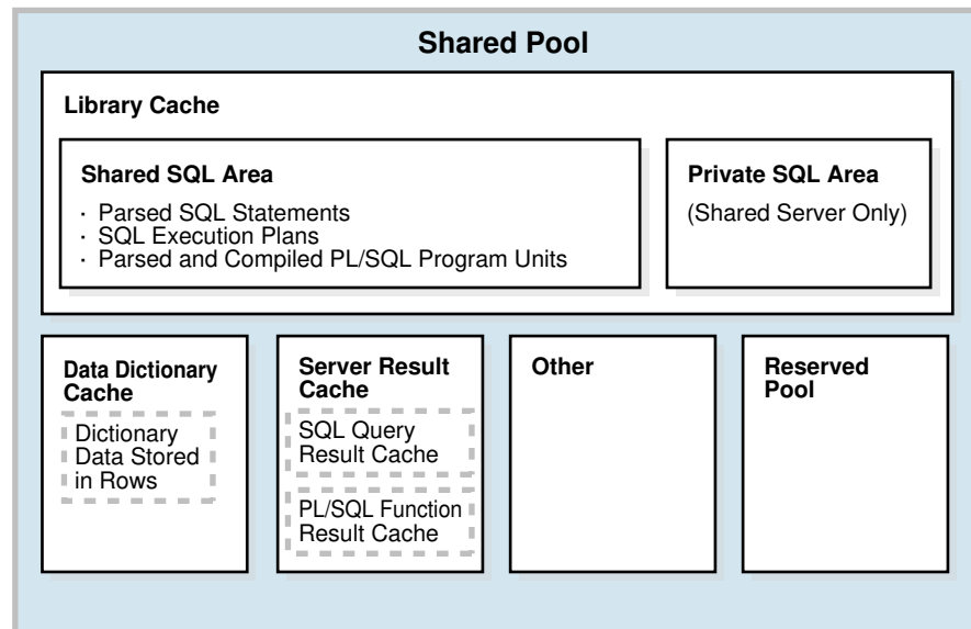
Figure 17-5 Shared Pool
