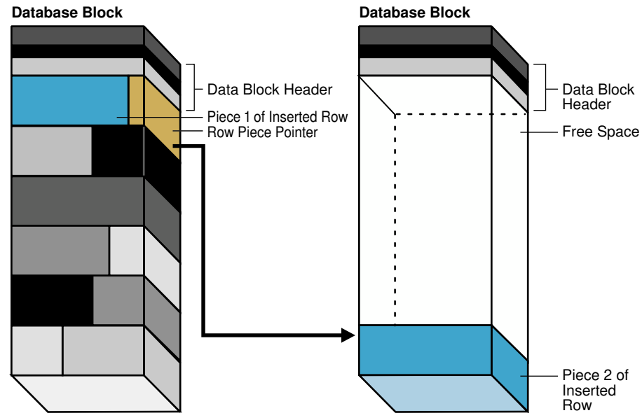
Figure 15-13 Row Chaining
