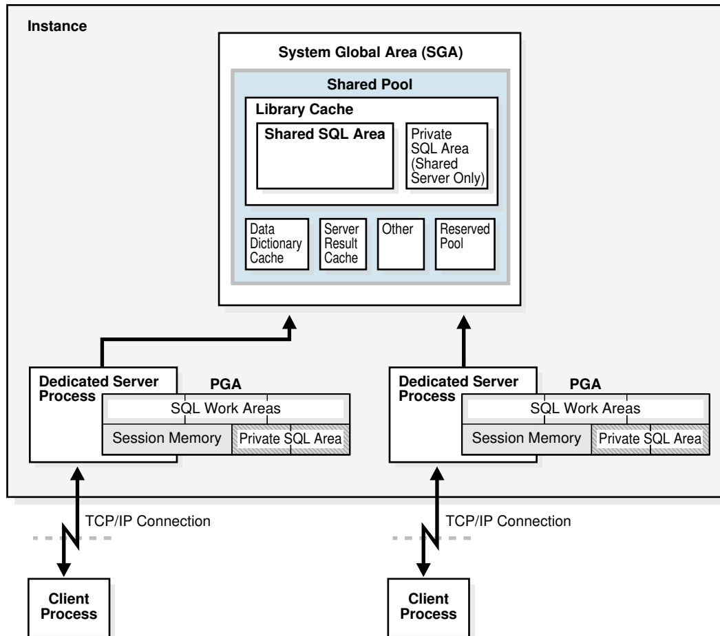
Figure 19-8 Oracle Database Using Dedicated Server Processes
