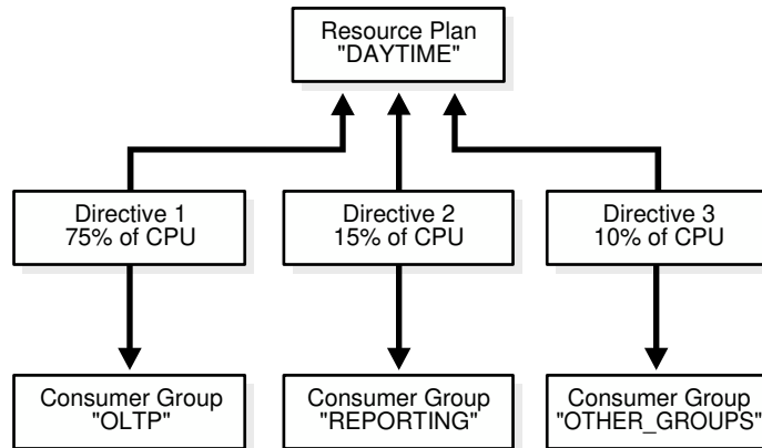
Figure 22-7 Simple Resource Plan
