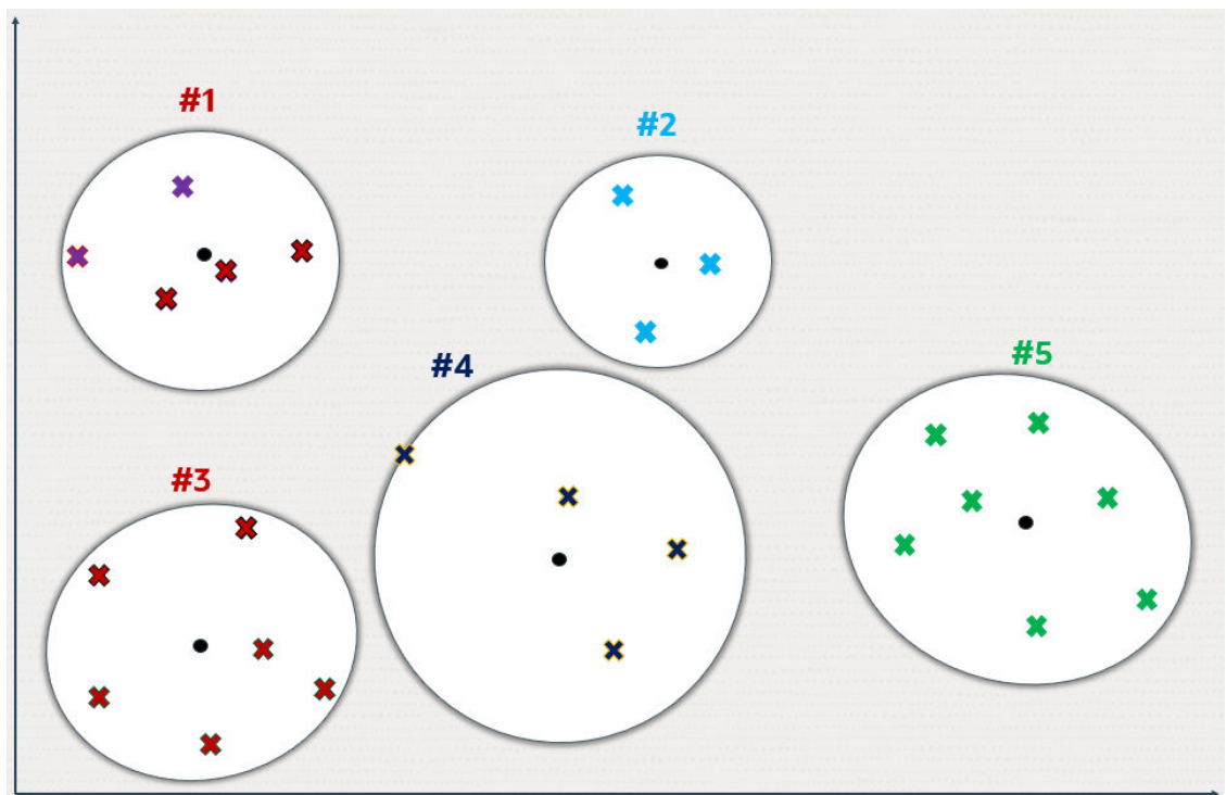
Figure 21-6 Inverted File Flat Index Using 2D
