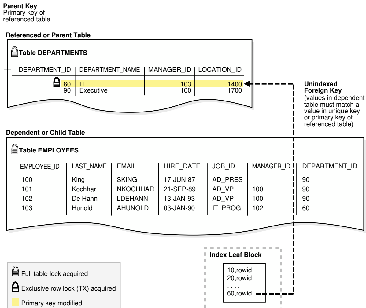
Figure 12-3 Locking Mechanisms with Unindexed Foreign Key
