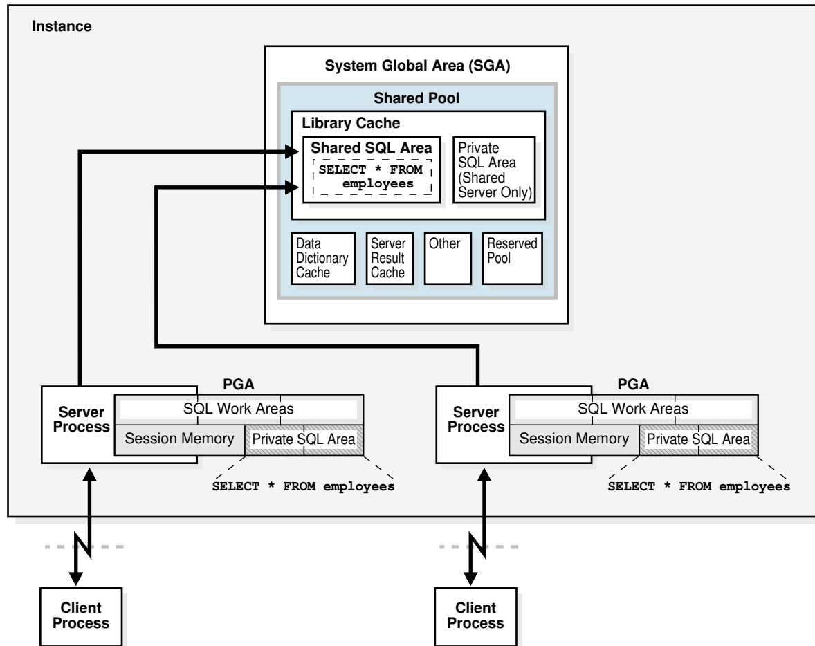
Figure 17-6 Private SQL Areas and Shared SQL Area
