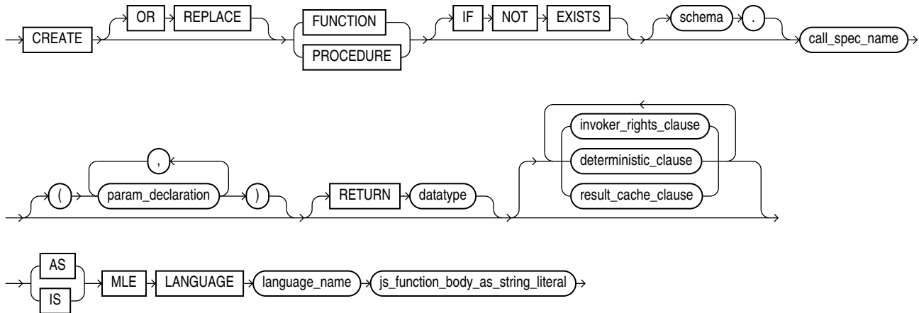
Figure 5-5 MLE Inline Call Specification Syntax
