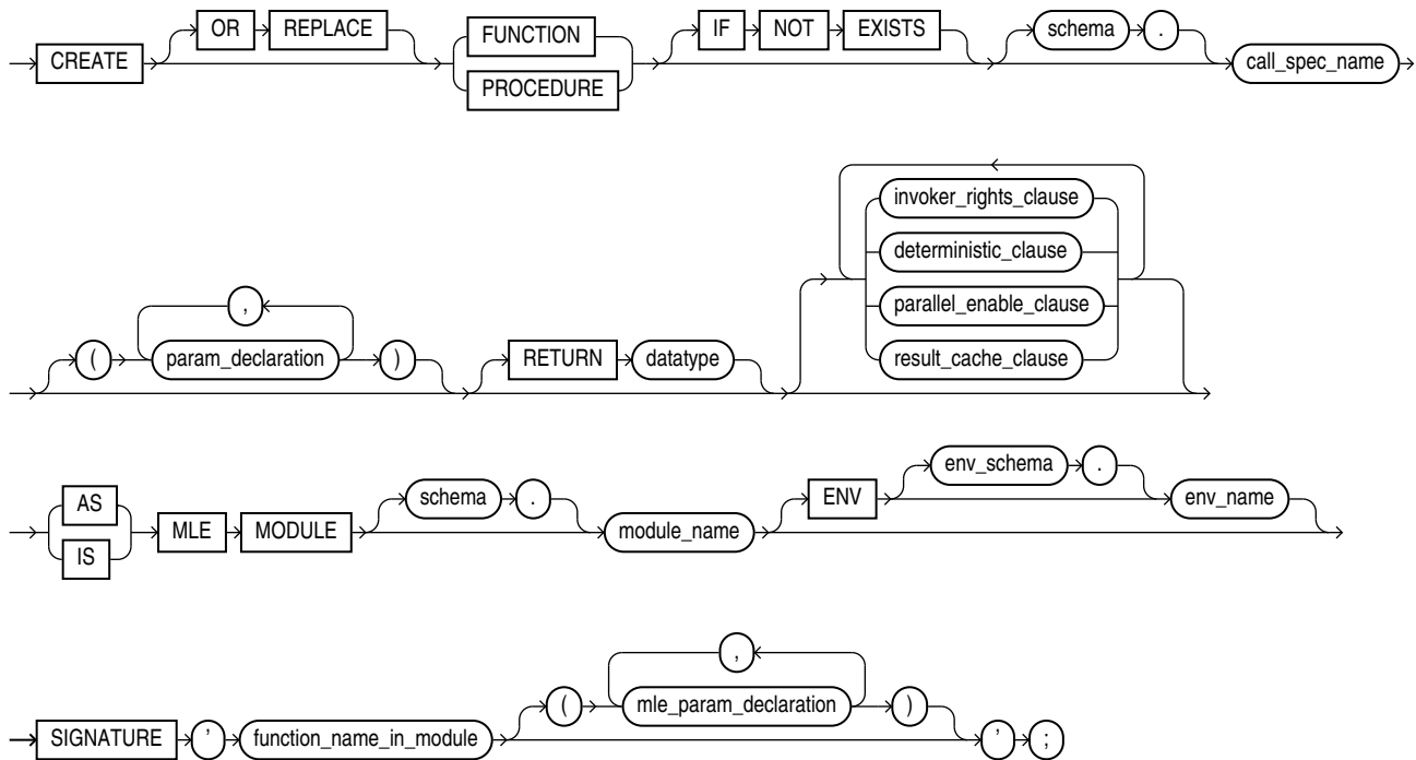
Figure 5-1 MLE Call Specification Syntax
