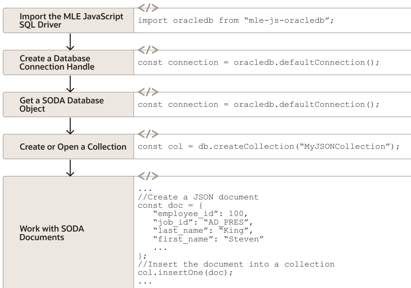
Figure 7-1 SODA for In-Database JavaScript Basic Workflow
