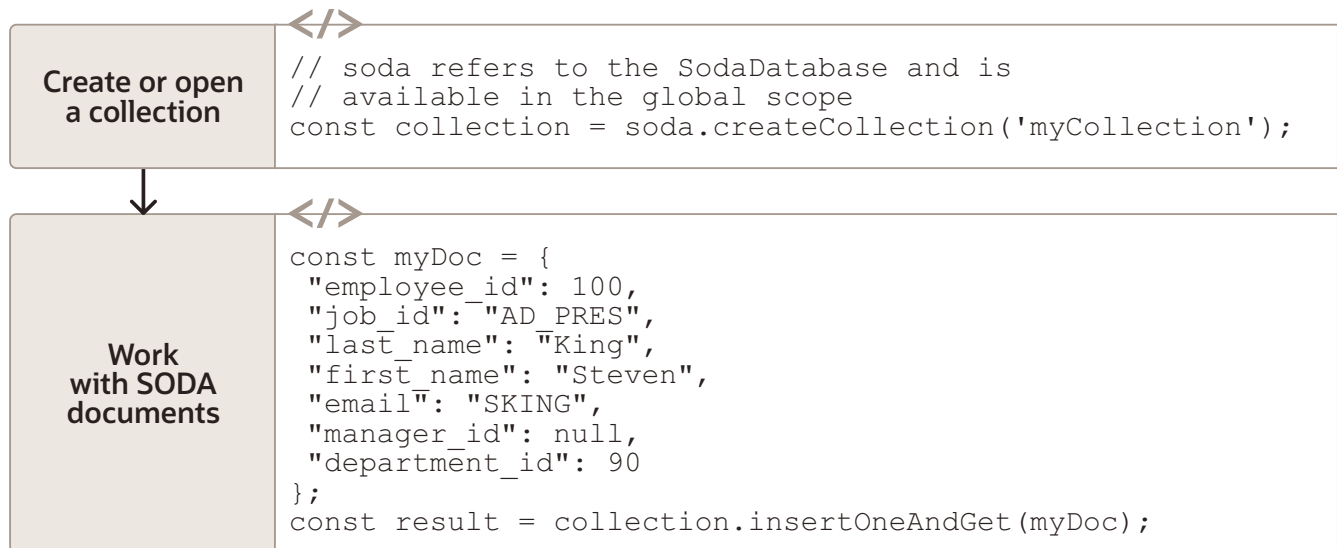
Figure 7-2 SODA for In-Database JavaScript Simplified Workflow
