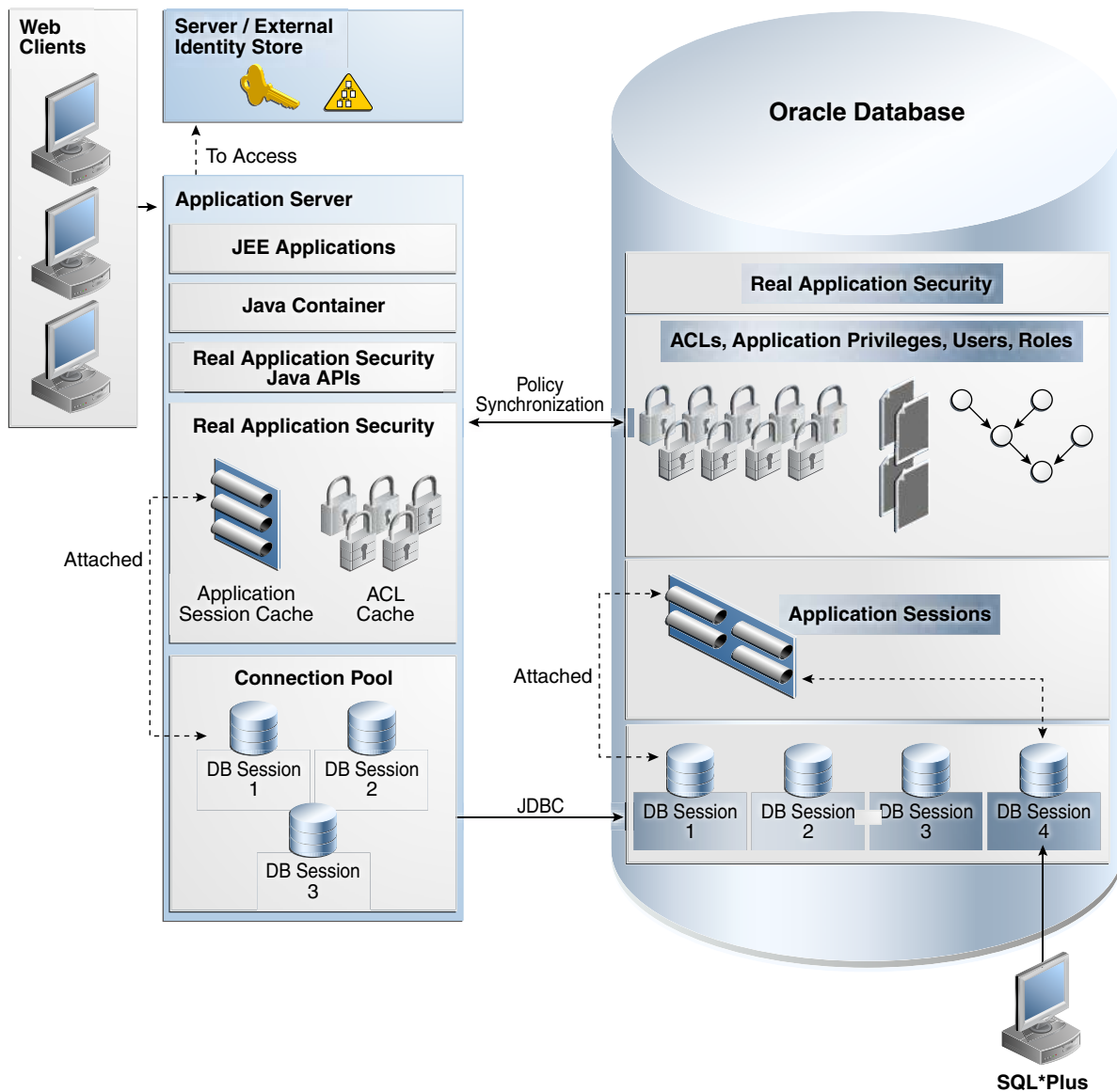
Figure 3-1 Real Application Security Architecture
